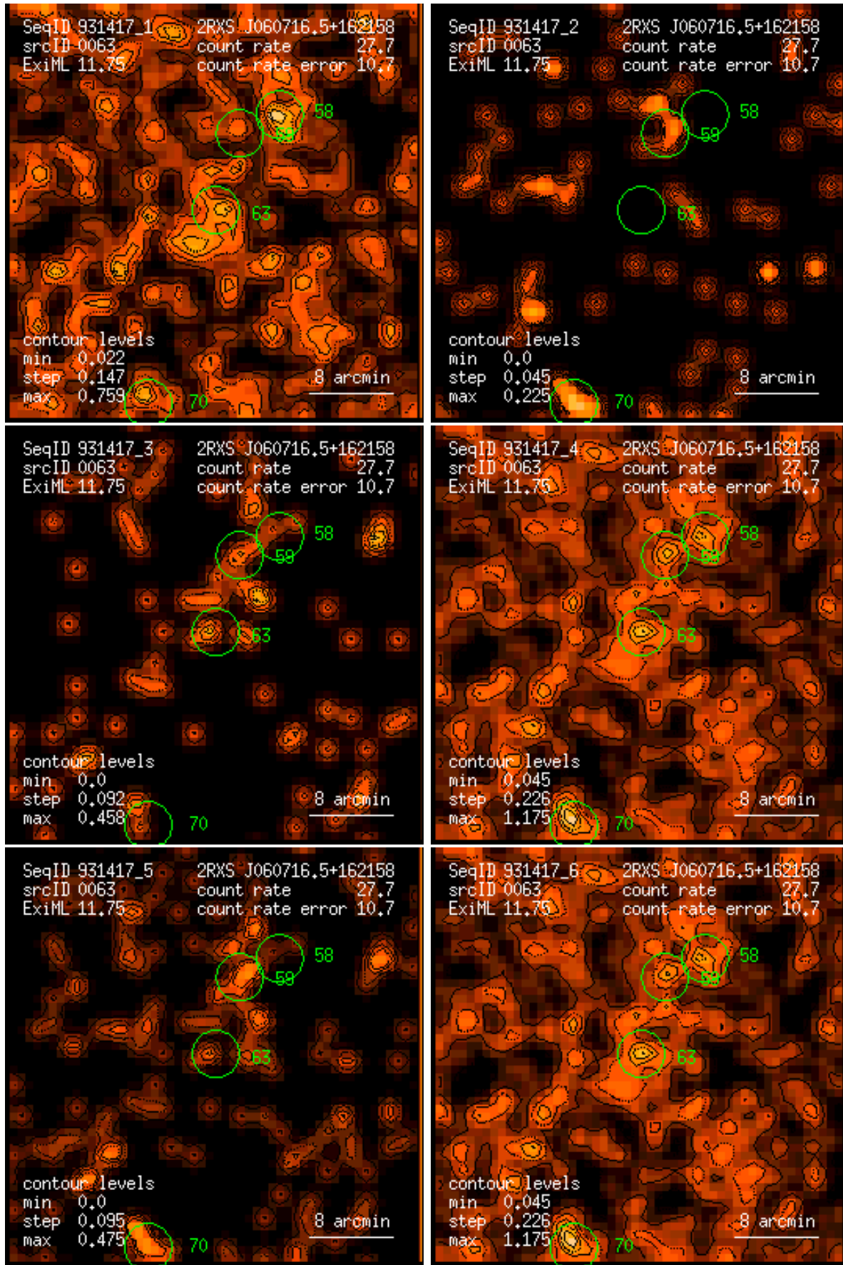
Figure 63: RASS 931417: detection 0063: band rate images, Gaussian filter: (1) PSPC channels 11 – 41, (2) 52 – 90, (3) 91 – 201, (4) 11 – 235, (5) 52 – 201, (6) 11 – 201. Broad band rates in counts/ks. Band rate contour levels in counts/ks/arcmin 2 .
