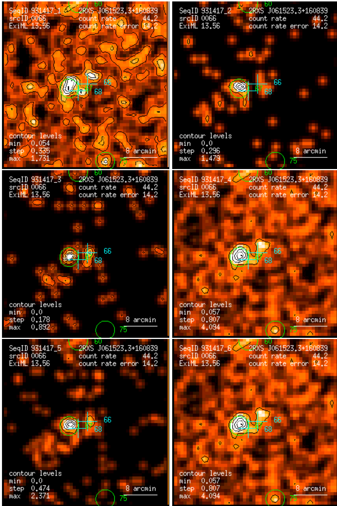
Figure 66: RASS 931417: detection 0066: band rate images, Gaussian filter: (1) PSPC channels 11 – 41, (2) 52 – 90, (3) 91 – 201, (4) 11 – 235, (5) 52 – 201, (6) 11 – 201. Broad band rates in counts/ks. Band rate contour levels in counts/ks/arcmin 2 .
