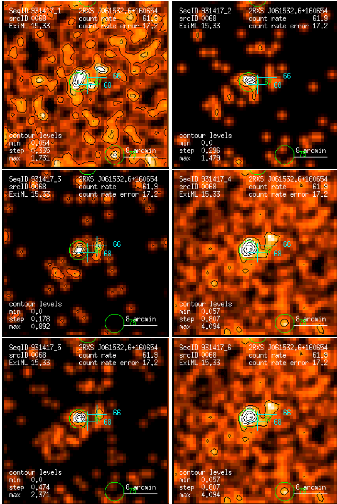
Figure 68: RASS 931417: detection 0068: band rate images, Gaussian filter: (1) PSPC channels 11 – 41, (2) 52 – 90, (3) 91 – 201, (4) 11 – 235, (5) 52 – 201, (6) 11 – 201. Broad band rates in counts/ks. Band rate contour levels in counts/ks/arcmin 2 .
