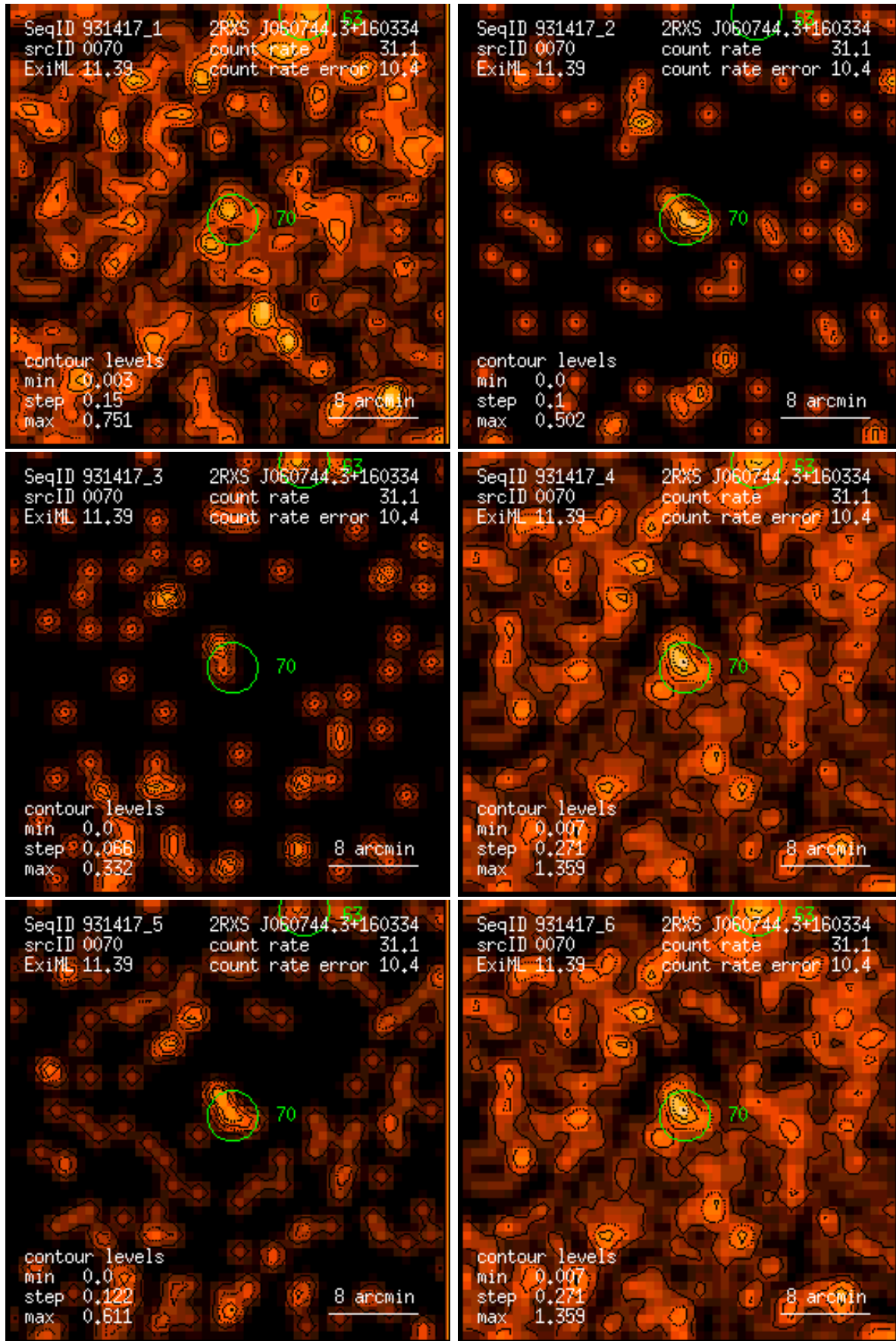
Figure 70: RASS 931417: detection 0070: band rate images, Gaussian filter: (1) PSPC channels 11 – 41, (2) 52 – 90, (3) 91 – 201, (4) 11 – 235, (5) 52 – 201, (6) 11 – 201. Broad band rates in counts/ks. Band rate contour levels in counts/ks/arcmin 2 .
