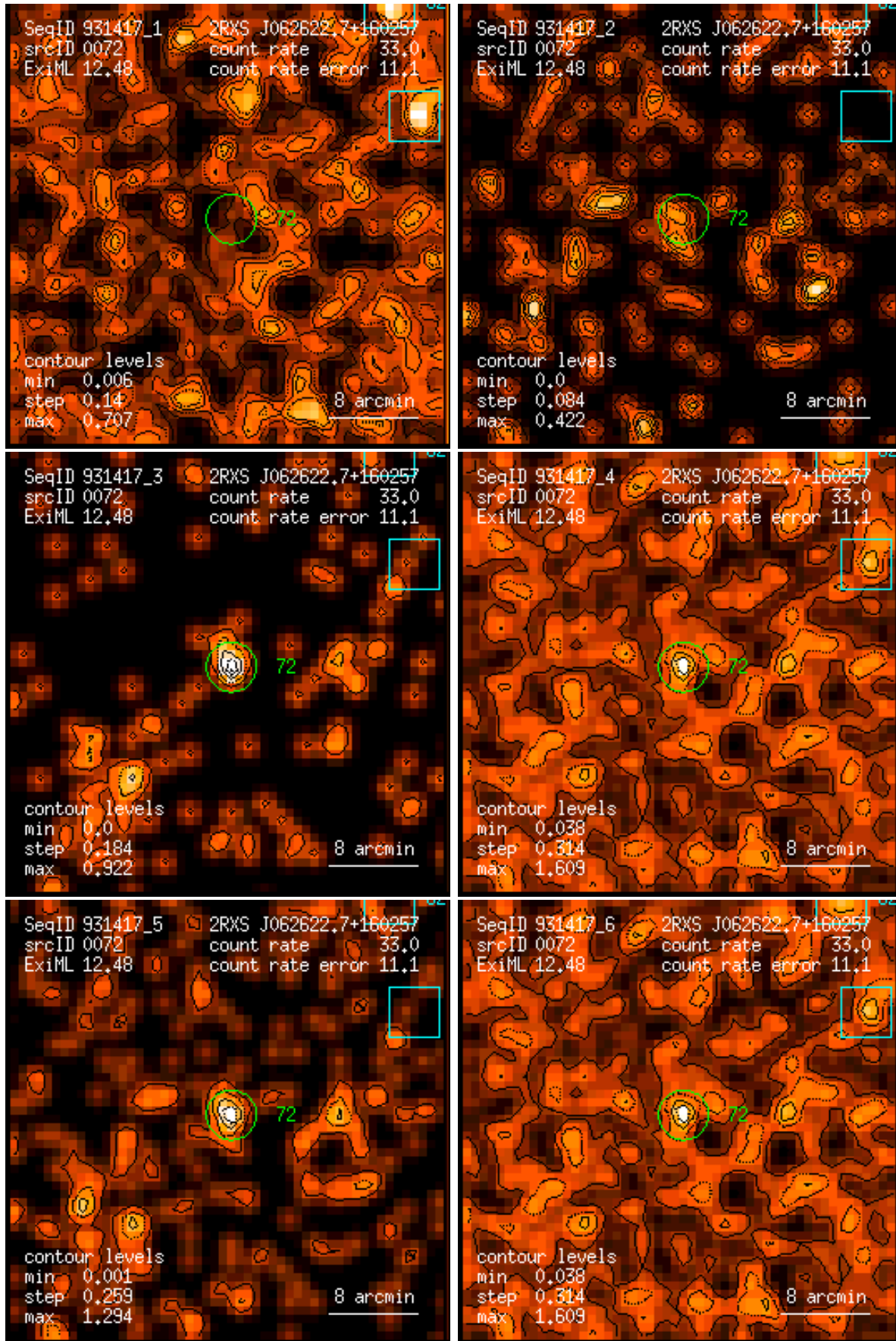
Figure 72: RASS 931417: detection 0072: band rate images, Gaussian filter: (1) PSPC channels 11 – 41, (2) 52 – 90, (3) 91 – 201, (4) 11 – 235, (5) 52 – 201, (6) 11 – 201. Broad band rates in counts/ks. Band rate contour levels in counts/ks/arcmin 2 .
