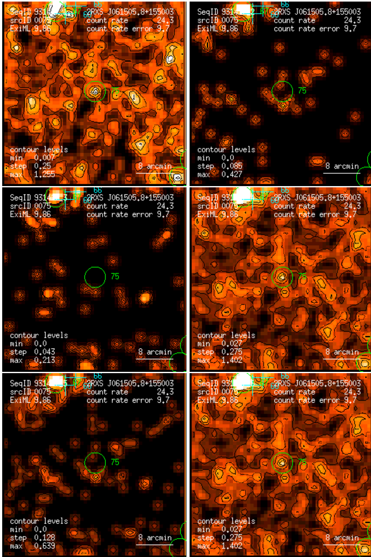
Figure 75: RASS 931417: detection 0075: band rate images, Gaussian filter: (1) PSPC channels 11 – 41, (2) 52 – 90, (3) 91 – 201, (4) 11 – 235, (5) 52 – 201, (6) 11 – 201. Broad band rates in counts/ks. Band rate contour levels in counts/ks/arcmin 2 .
