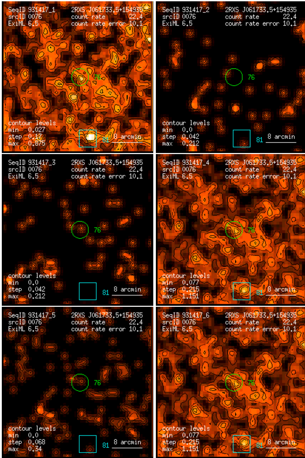
Figure 76: RASS 931417: detection 0076: band rate images, Gaussian filter: (1) PSPC channels 11 – 41, (2) 52 – 90, (3) 91 – 201, (4) 11 – 235, (5) 52 – 201, (6) 11 – 201. Broad band rates in counts/ks. Band rate contour levels in counts/ks/arcmin 2 .
