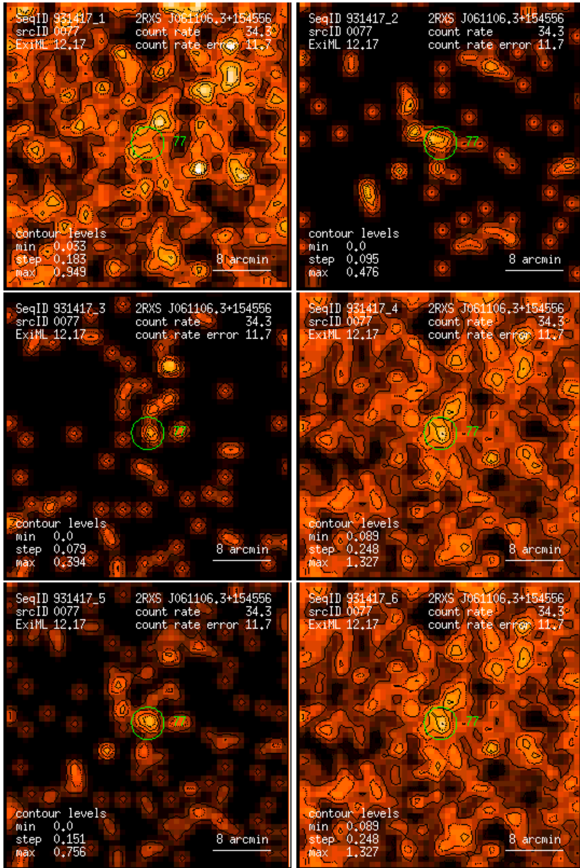
Figure 77: RASS 931417: detection 0077: band rate images, Gaussian filter: (1) PSPC channels 11 – 41, (2) 52 – 90, (3) 91 – 201, (4) 11 – 235, (5) 52 – 201, (6) 11 – 201. Broad band rates in counts/ks. Band rate contour levels in counts/ks/arcmin 2 .
