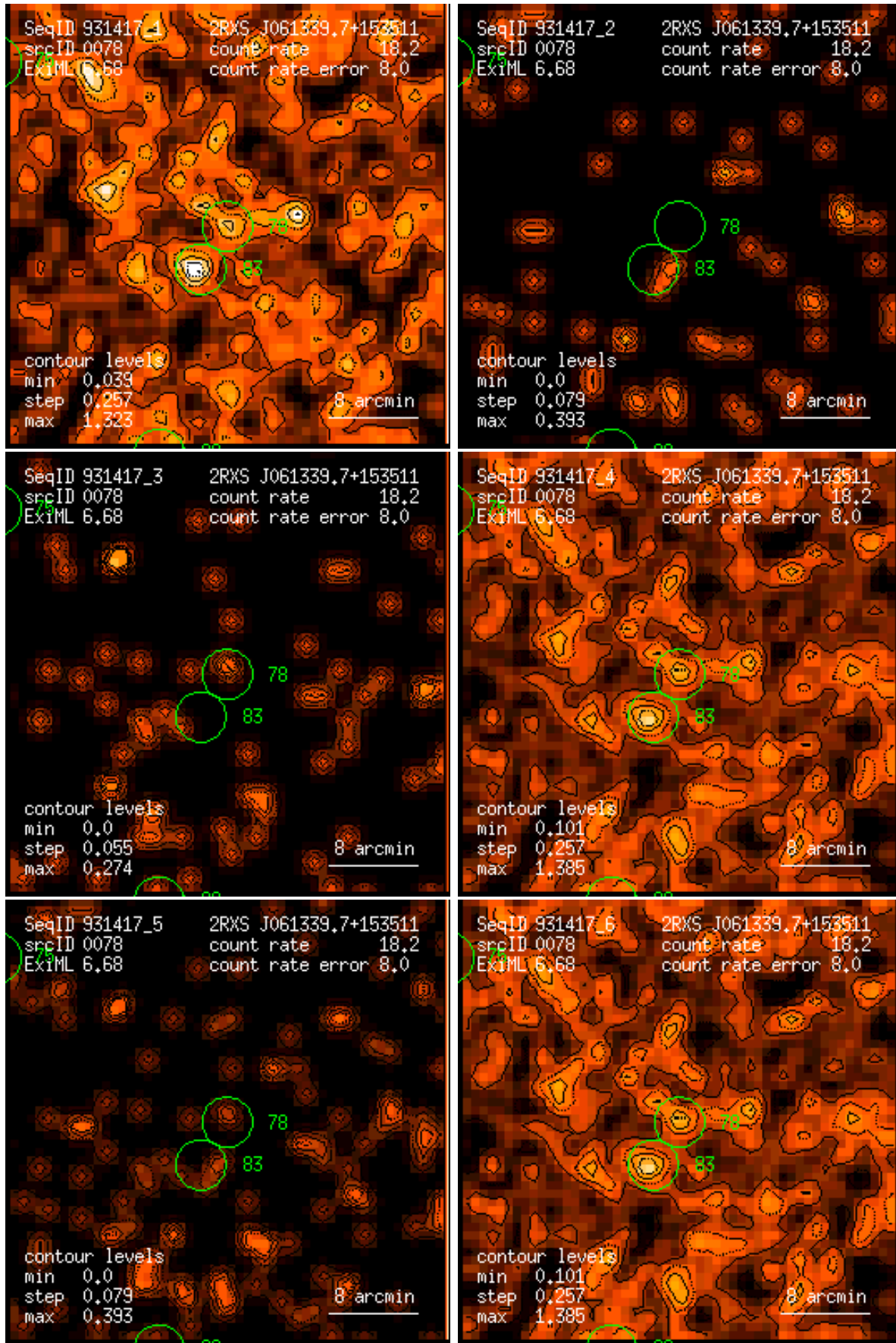
Figure 78: RASS 931417: detection 0078: band rate images, Gaussian filter: (1) PSPC channels 11 – 41, (2) 52 – 90, (3) 91 – 201, (4) 11 – 235, (5) 52 – 201, (6) 11 – 201. Broad band rates in counts/ks. Band rate contour levels in counts/ks/arcmin 2 .
