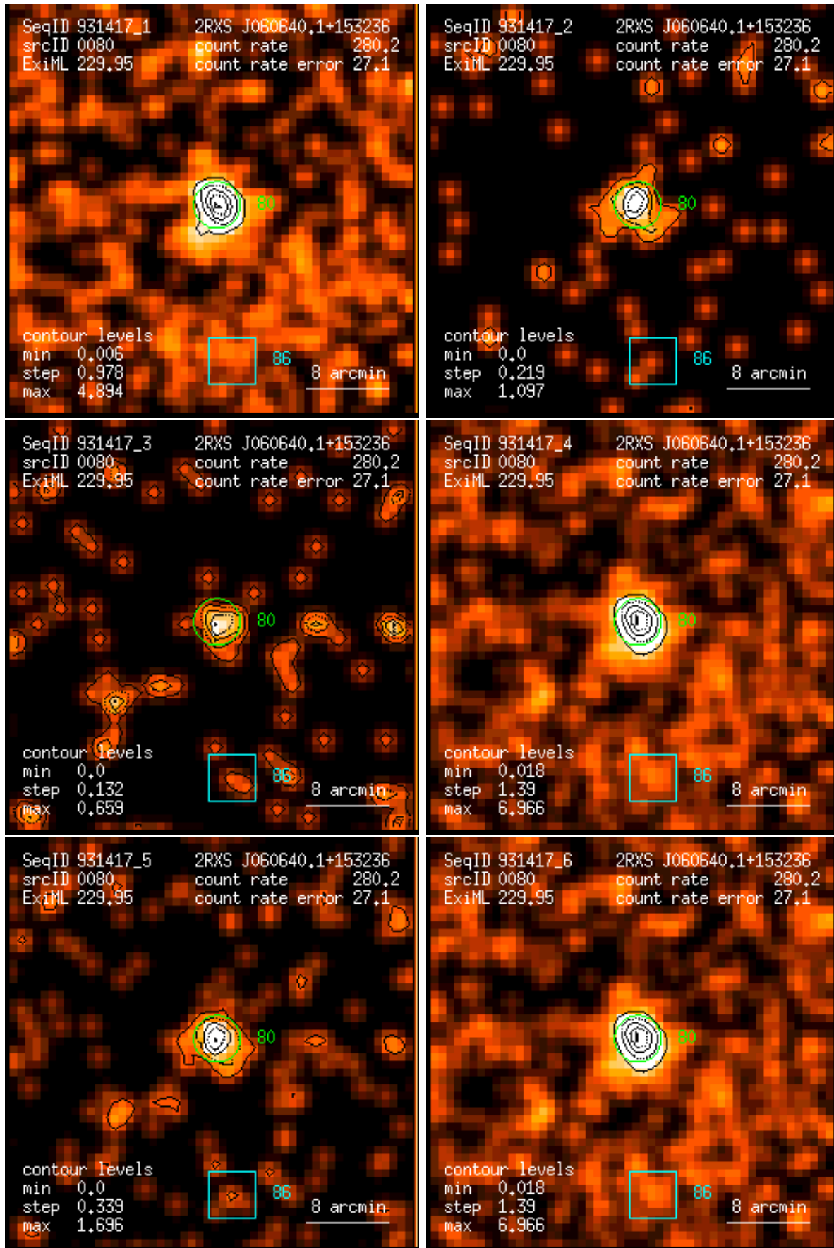
Figure 80: RASS 931417: detection 0080: band rate images, Gaussian filter: (1) PSPC channels 11 – 41, (2) 52 – 90, (3) 91 – 201, (4) 11 – 235, (5) 52 – 201, (6) 11 – 201. Broad band rates in counts/ks. Band rate contour levels in counts/ks/arcmin 2 .
