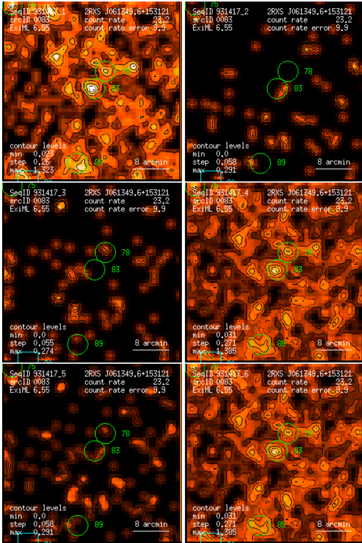
Figure 83: RASS 931417: detection 0083: band rate images, Gaussian filter: (1) PSPC channels 11 – 41, (2) 52 – 90, (3) 91 – 201, (4) 11 – 235, (5) 52 – 201, (6) 11 – 201. Broad band rates in counts/ks. Band rate contour levels in counts/ks/arcmin 2 .
