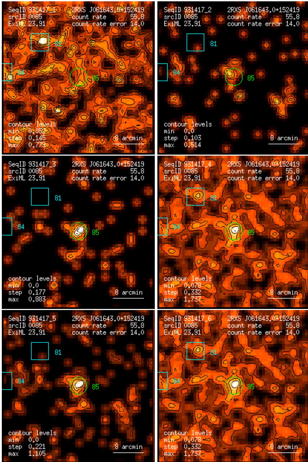
Figure 85: RASS 931417: detection 0085: band rate images, Gaussian filter: (1) PSPC channels 11 – 41, (2) 52 – 90, (3) 91 – 201, (4) 11 – 235, (5) 52 – 201, (6) 11 – 201. Broad band rates in counts/ks. Band rate contour levels in counts/ks/arcmin 2 .
