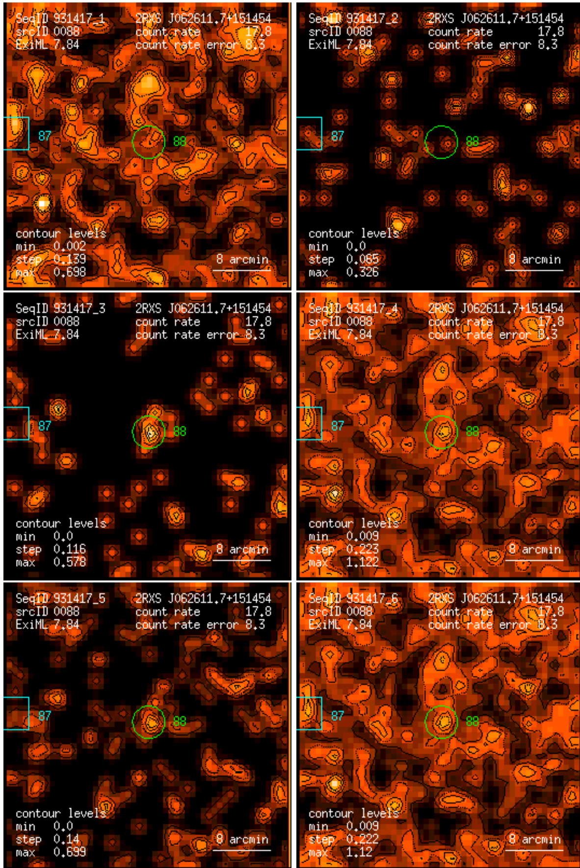
Figure 88: RASS 931417: detection 0088: band rate images, Gaussian filter: (1) PSPC channels 11 – 41, (2) 52 – 90, (3) 91 – 201, (4) 11 – 235, (5) 52 – 201, (6) 11 – 201. Broad band rates in counts/ks. Band rate contour levels in counts/ks/arcmin 2 .
