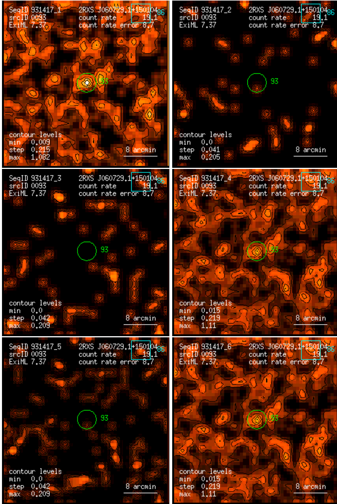
Figure 93: RASS 931417: detection 0093: band rate images, Gaussian filter: (1) PSPC channels 11 – 41, (2) 52 – 90, (3) 91 – 201, (4) 11 – 235, (5) 52 – 201, (6) 11 – 201. Broad band rates in counts/ks. Band rate contour levels in counts/ks/arcmin 2 .
