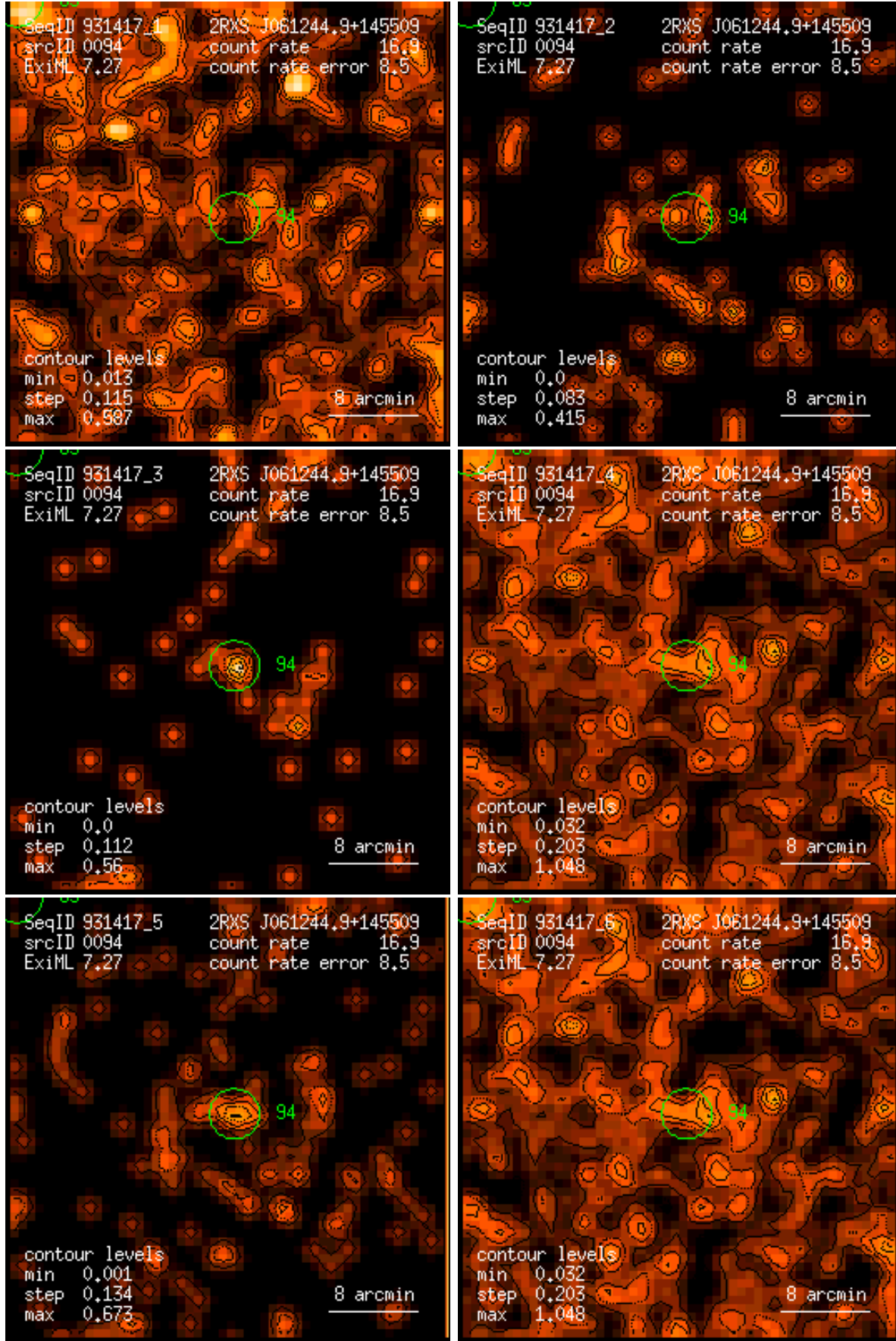
Figure 94: RASS 931417: detection 0094: band rate images, Gaussian filter: (1) PSPC channels 11 – 41, (2) 52 – 90, (3) 91 – 201, (4) 11 – 235, (5) 52 – 201, (6) 11 – 201. Broad band rates in counts/ks. Band rate contour levels in counts/ks/arcmin 2 .
