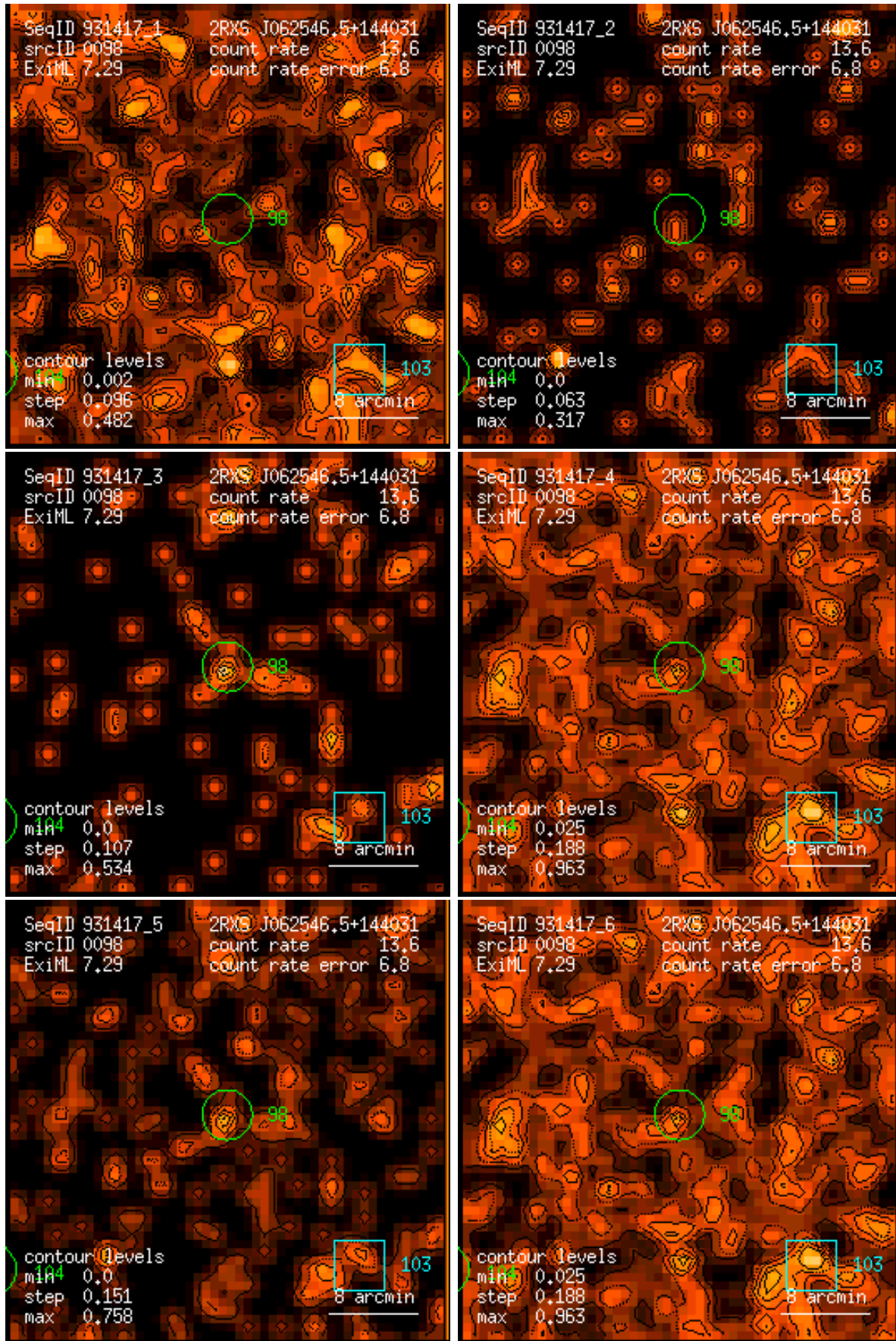
Figure 98: RASS 931417: detection 0098: band rate images, Gaussian filter: (1) PSPC channels 11 – 41, (2) 52 – 90, (3) 91 – 201, (4) 11 – 235, (5) 52 – 201, (6) 11 – 201. Broad band rates in counts/ks. Band rate contour levels in counts/ks/arcmin 2 .
