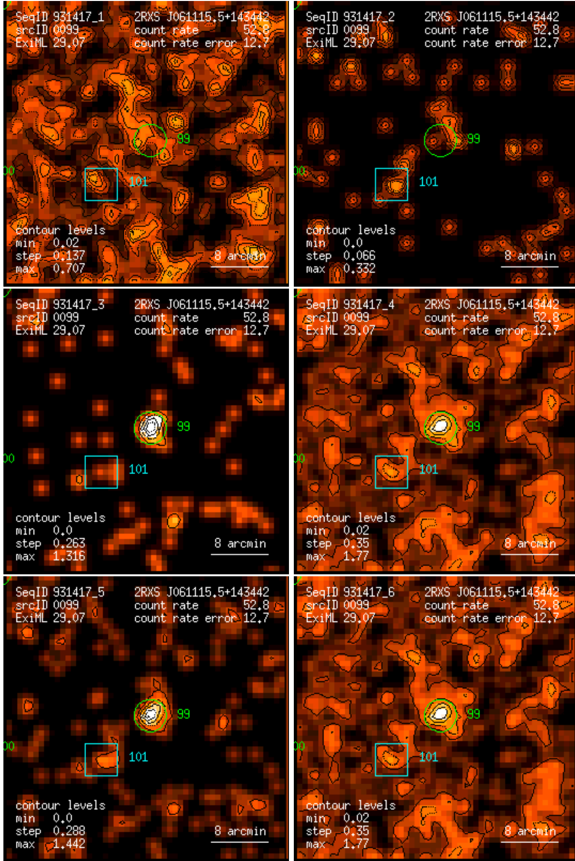
Figure 99: RASS 931417: detection 0099: band rate images, Gaussian filter: (1) PSPC channels 11 – 41, (2) 52 – 90, (3) 91 – 201, (4) 11 – 235, (5) 52 – 201, (6) 11 – 201. Broad band rates in counts/ks. Band rate contour levels in counts/ks/arcmin 2 .
