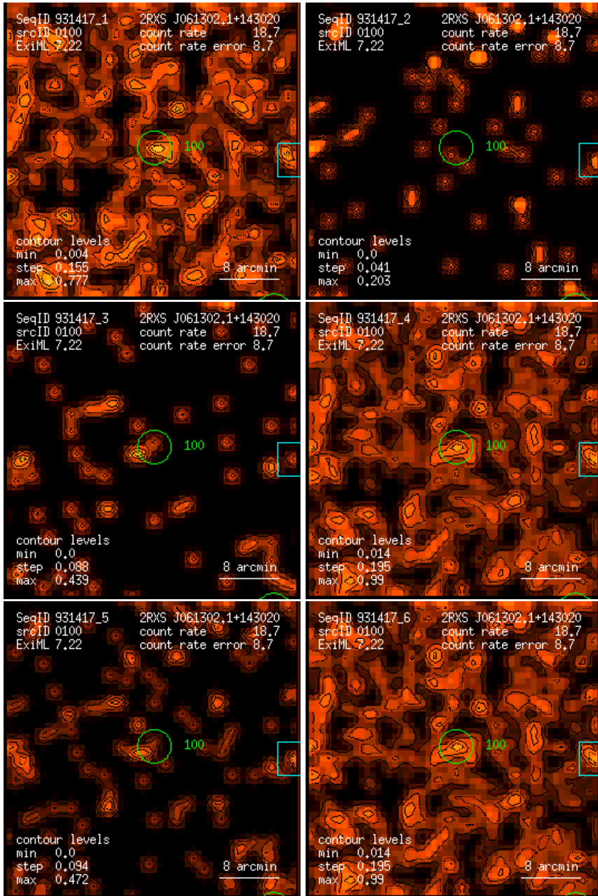
Figure 100: RASS 931417: detection 0100: band rate images, Gaussian filter: (1) PSPC channels 11 – 41, (2) 52 – 90, (3) 91 – 201, (4) 11 – 235, (5) 52 – 201, (6) 11 – 201. Broad band rates in counts/ks. Band rate contour levels in counts/ks/arcmin 2 .
