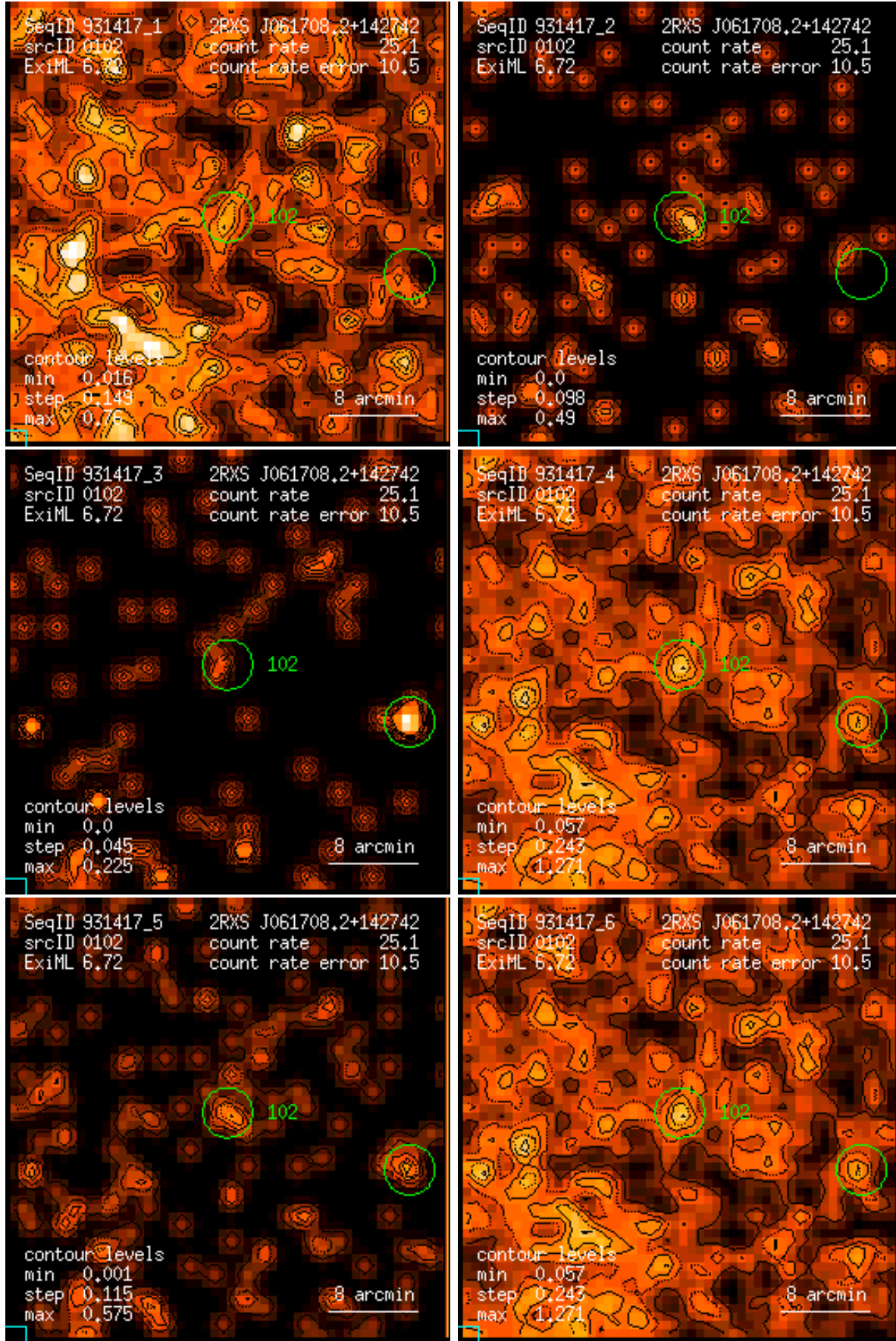
Figure 102: RASS 931417: detection 0102: band rate images, Gaussian filter: (1) PSPC channels 11 – 41, (2) 52 – 90, (3) 91 – 201, (4) 11 – 235, (5) 52 – 201, (6) 11 – 201. Broad band rates in counts/ks. Band rate contour levels in counts/ks/arcmin 2 .
