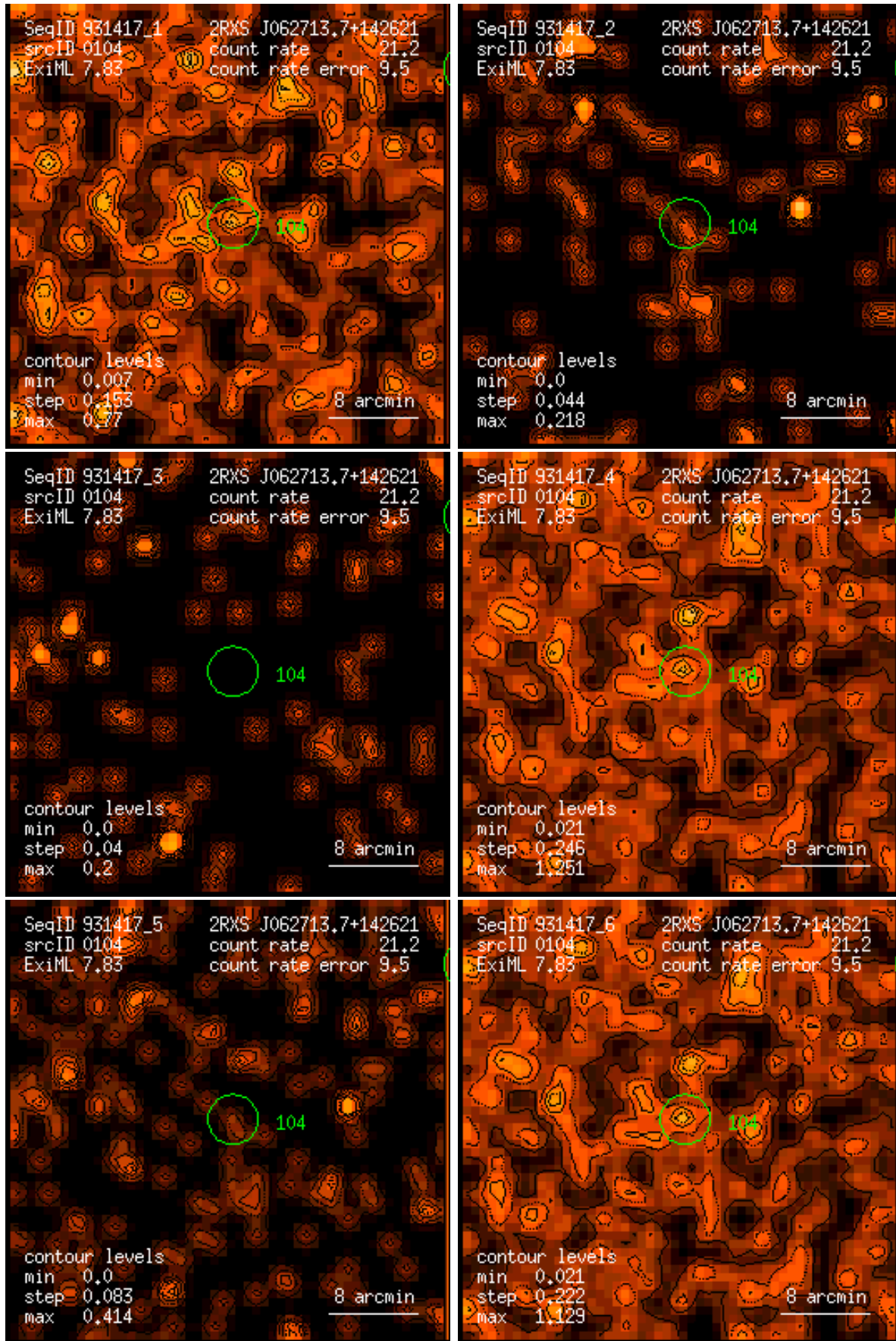
Figure 104: RASS 931417: detection 0104: band rate images, Gaussian filter: (1) PSPC channels 11 – 41, (2) 52 – 90, (3) 91 – 201, (4) 11 – 235, (5) 52 – 201, (6) 11 – 201. Broad band rates in counts/ks. Band rate contour levels in counts/ks/arcmin 2 .
