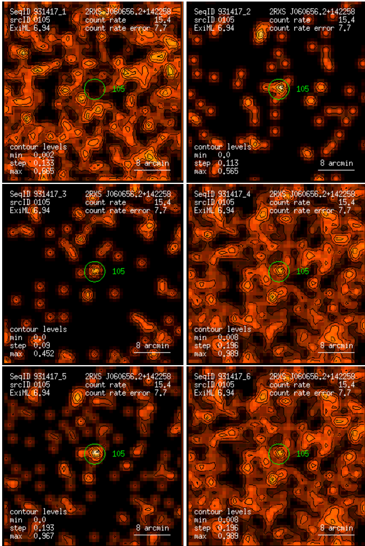
Figure 105: RASS 931417: detection 0105: band rate images, Gaussian filter: (1) PSPC channels 11 – 41, (2) 52 – 90, (3) 91 – 201, (4) 11 – 235, (5) 52 – 201, (6) 11 – 201. Broad band rates in counts/ks. Band rate contour levels in counts/ks/arcmin 2 .
