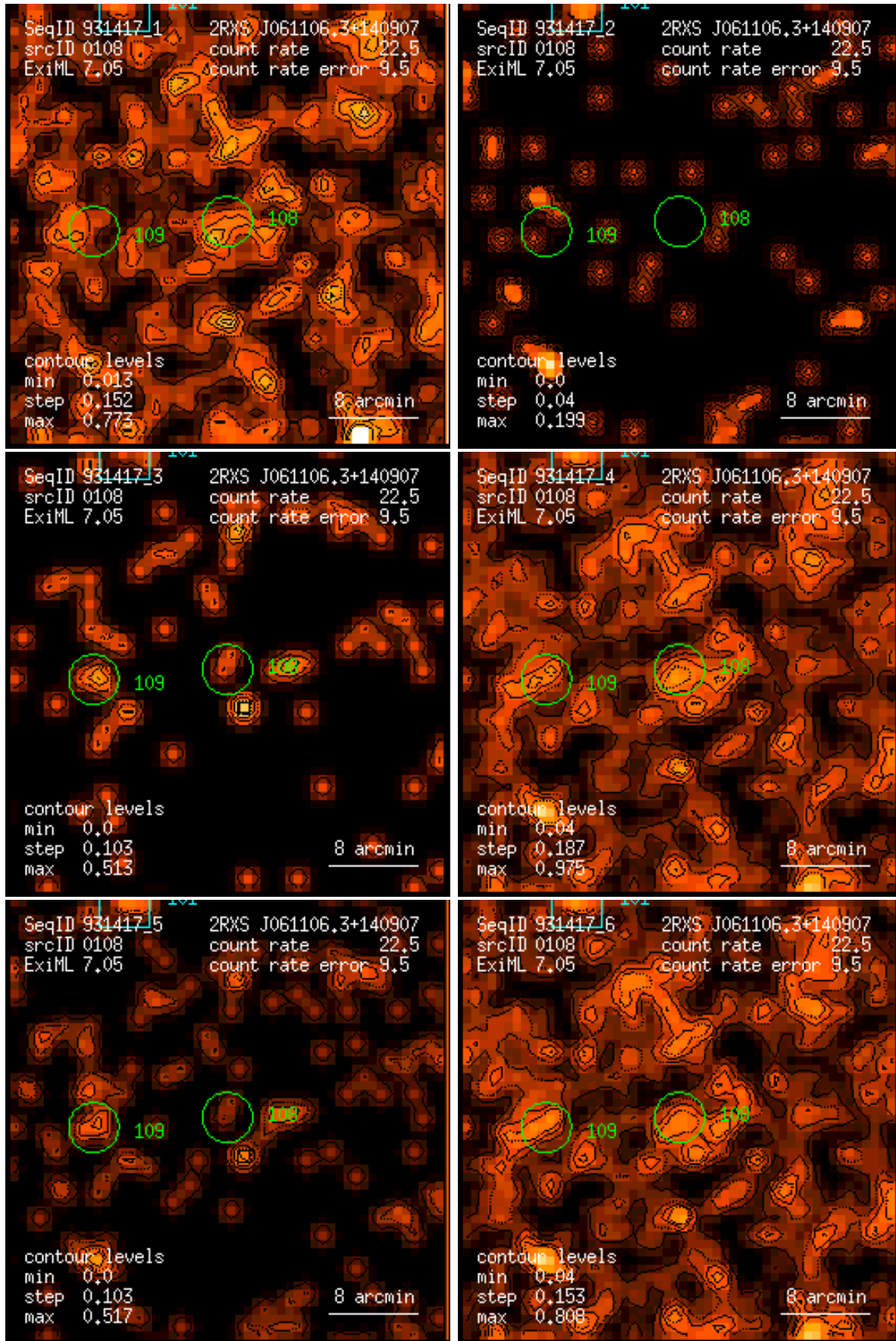
Figure 108: RASS 931417: detection 0108: band rate images, Gaussian filter: (1) PSPC channels 11 – 41, (2) 52 – 90, (3) 91 – 201, (4) 11 – 235, (5) 52 – 201, (6) 11 – 201. Broad band rates in counts/ks. Band rate contour levels in counts/ks/arcmin 2 .
