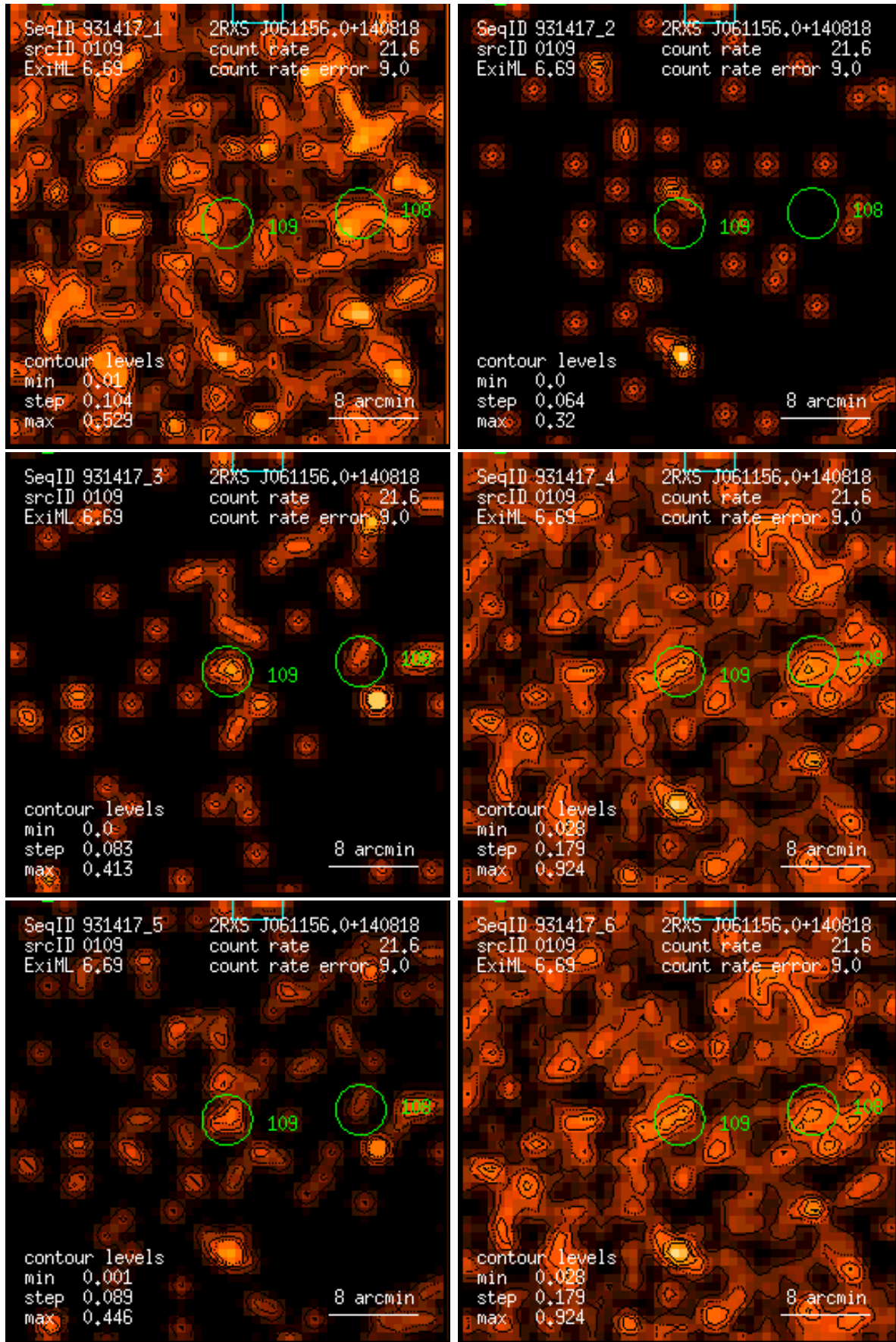
Figure 109: RASS 931417: detection 0109: band rate images, Gaussian filter: (1) PSPC channels 11 – 41, (2) 52 – 90, (3) 91 – 201, (4) 11 – 235, (5) 52 – 201, (6) 11 – 201. Broad band rates in counts/ks. Band rate contour levels in counts/ks/arcmin 2 .
