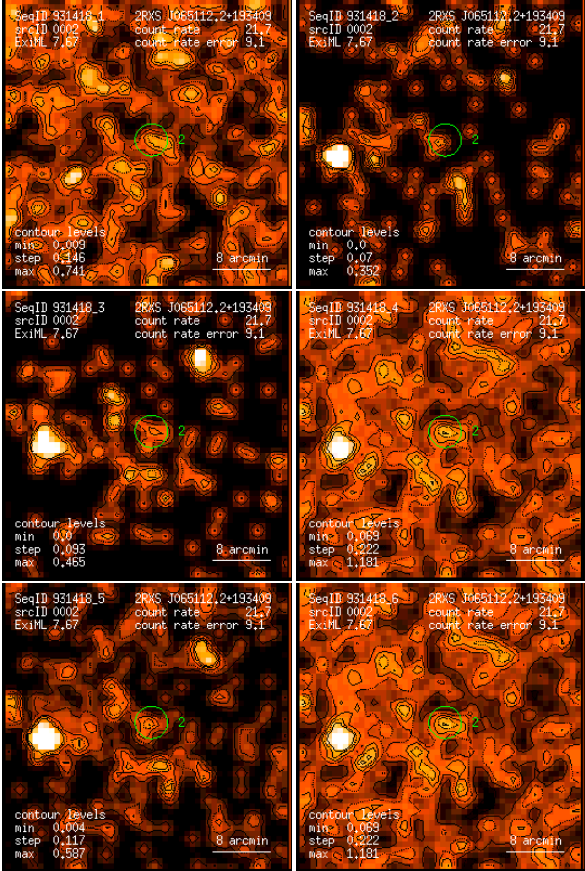
Figure 2: RASS 931418: detection 0002: band rate images, Gaussian filter: (1) PSPC channels 11 – 41, (2) 52 – 90, (3) 91 – 201, (4) 11 – 235, (5) 52 – 201, (6) 11 – 201. Broad band rates in counts/ks. Band rate contour levels in counts/ks/arcmin 2 .
