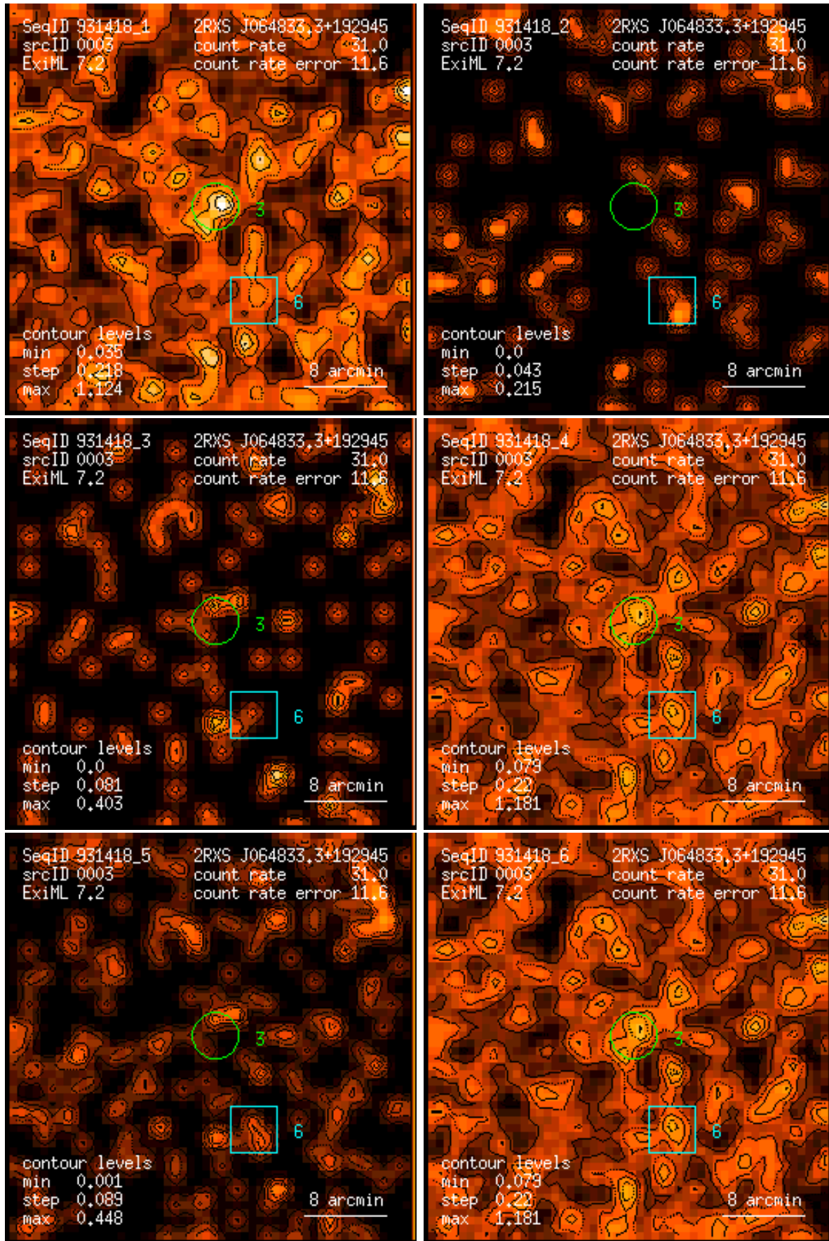
Figure 3: RASS 931418: detection 0003: band rate images, Gaussian filter: (1) PSPC channels 11 – 41, (2) 52 – 90, (3) 91 – 201, (4) 11 – 235, (5) 52 – 201, (6) 11 – 201. Broad band rates in counts/ks. Band rate contour levels in counts/ks/arcmin 2 .
