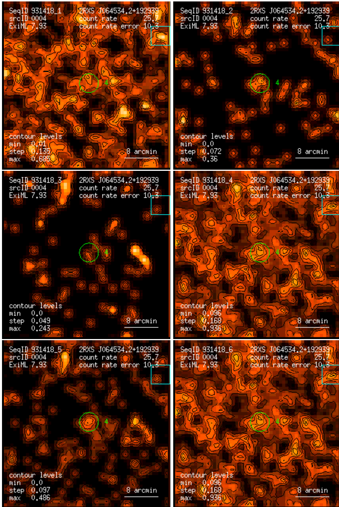
Figure 4: RASS 931418: detection 0004: band rate images, Gaussian filter: (1) PSPC channels 11 – 41, (2) 52 – 90, (3) 91 – 201, (4) 11 – 235, (5) 52 – 201, (6) 11 – 201. Broad band rates in counts/ks. Band rate contour levels in counts/ks/arcmin 2 .
