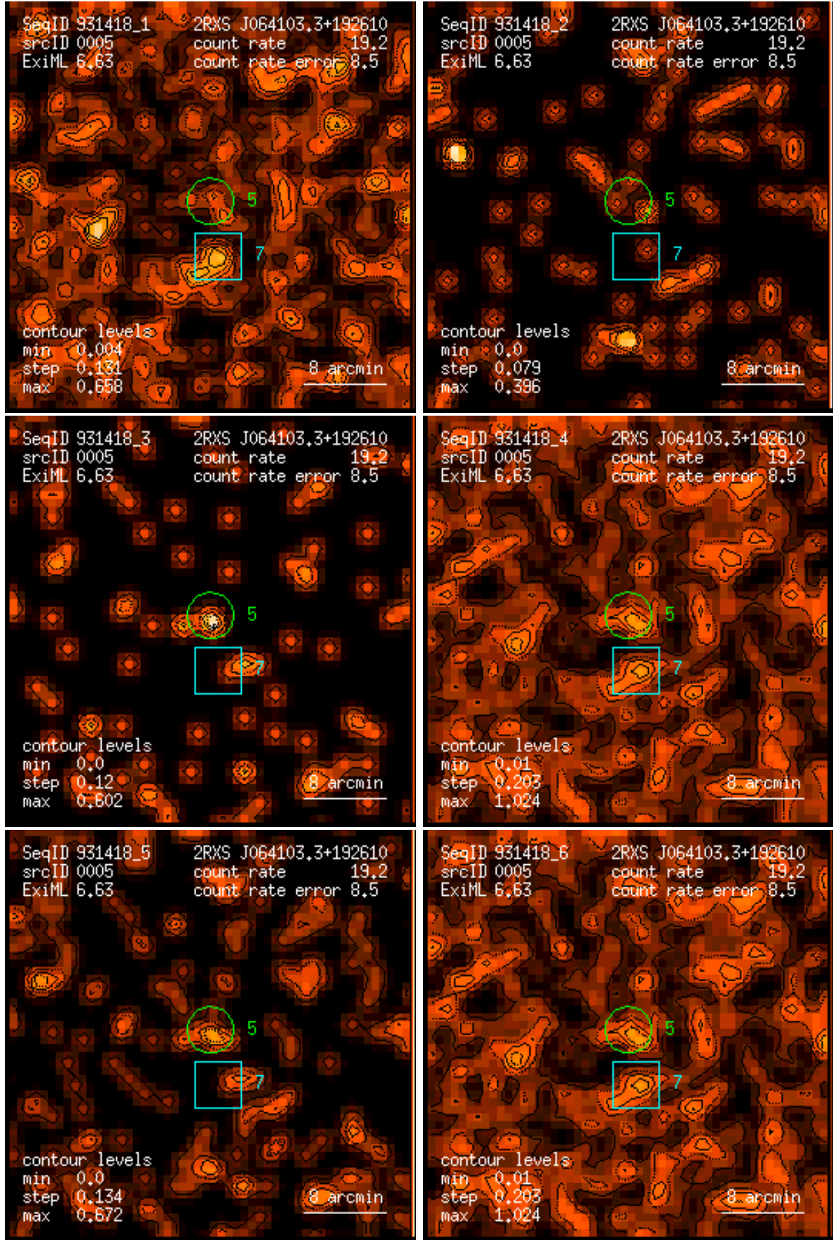
Figure 5: RASS 931418: detection 0005: band rate images, Gaussian filter: (1) PSPC channels 11 – 41, (2) 52 – 90, (3) 91 – 201, (4) 11 – 235, (5) 52 – 201, (6) 11 – 201. Broad band rates in counts/ks. Band rate contour levels in counts/ks/arcmin 2 .
