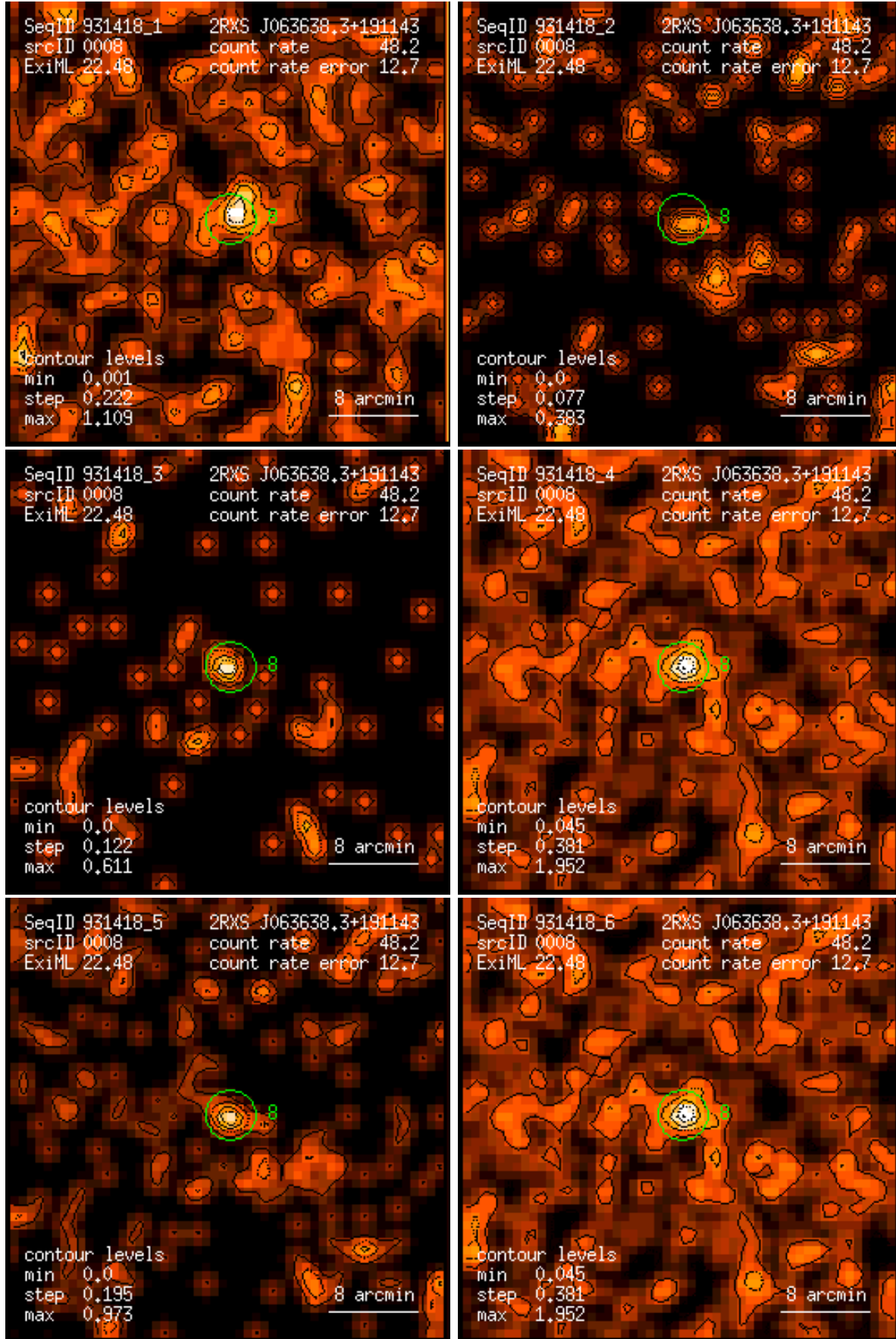
Figure 8: RASS 931418: detection 0008: band rate images, Gaussian filter: (1) PSPC channels 11 – 41, (2) 52 – 90, (3) 91 – 201, (4) 11 – 235, (5) 52 – 201, (6) 11 – 201. Broad band rates in counts/ks. Band rate contour levels in counts/ks/arcmin 2 .
