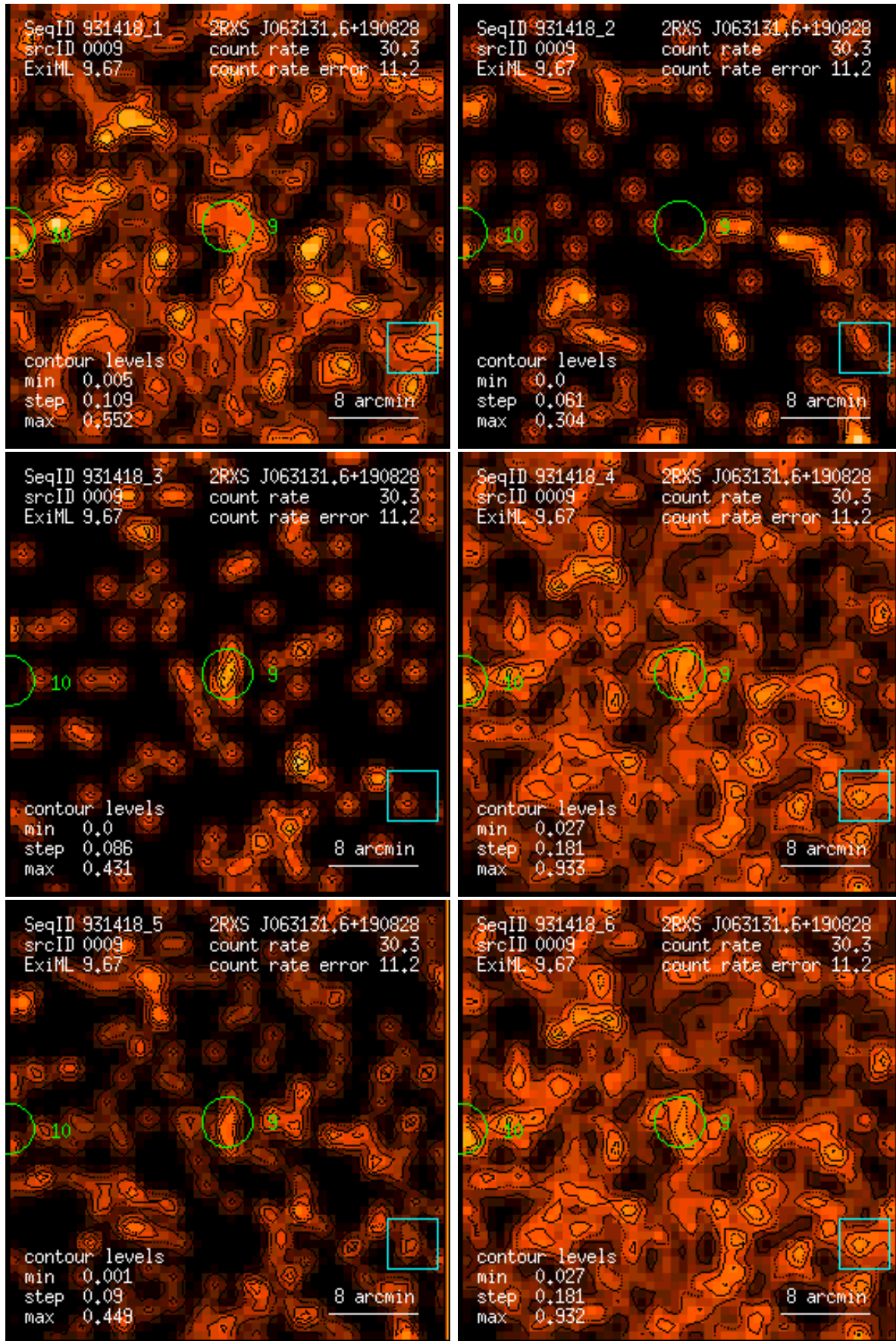
Figure 9: RASS 931418: detection 0009: band rate images, Gaussian filter: (1) PSPC channels 11 – 41, (2) 52 – 90, (3) 91 – 201, (4) 11 – 235, (5) 52 – 201, (6) 11 – 201. Broad band rates in counts/ks. Band rate contour levels in counts/ks/arcmin 2 .
