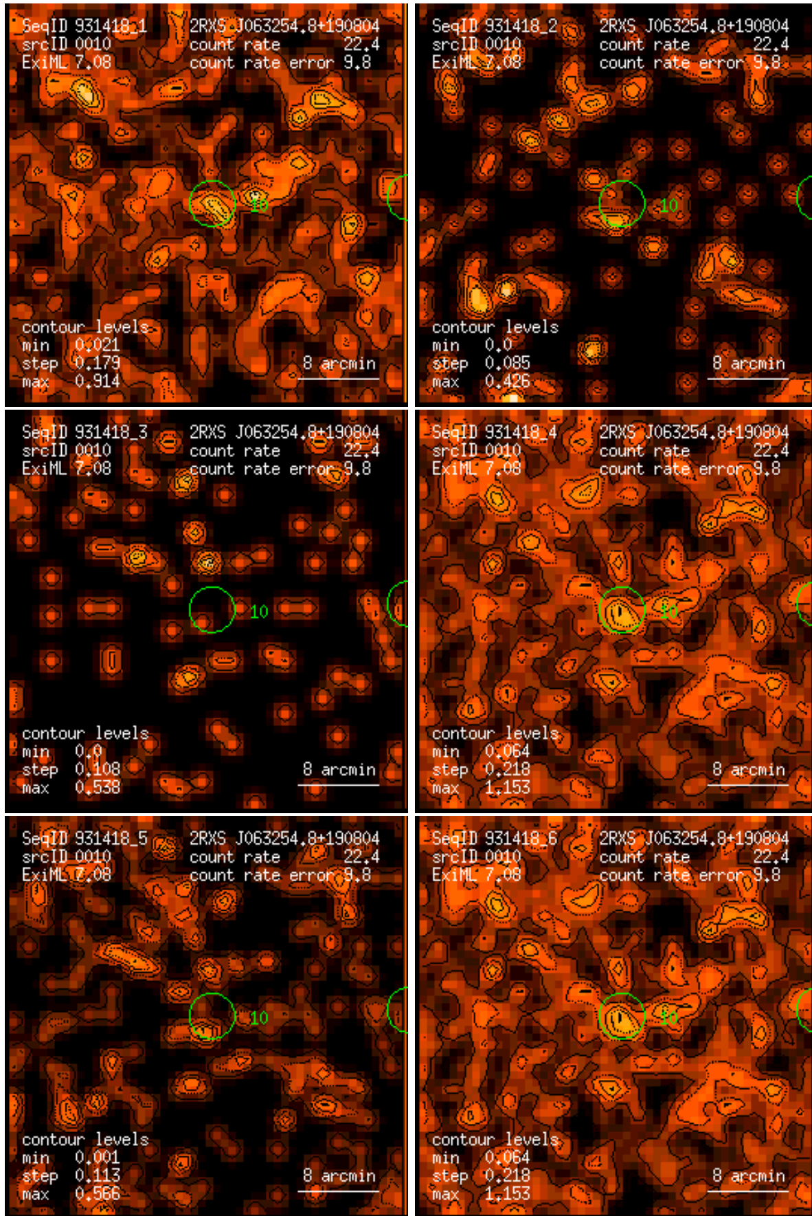
Figure 10: RASS 931418: detection 0010: band rate images, Gaussian filter: (1) PSPC channels 11 – 41, (2) 52 – 90, (3) 91 – 201, (4) 11 – 235, (5) 52 – 201, (6) 11 – 201. Broad band rates in counts/ks. Band rate contour levels in counts/ks/arcmin 2 .
