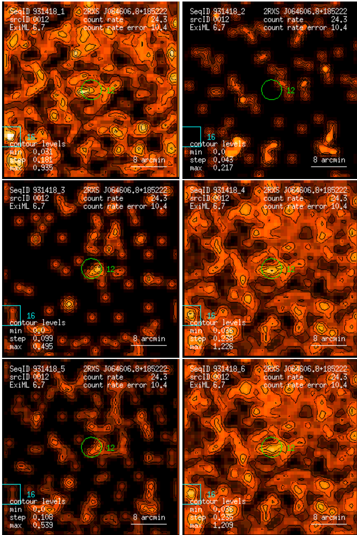
Figure 12: RASS 931418: detection 0012: band rate images, Gaussian filter: (1) PSPC channels 11 – 41, (2) 52 – 90, (3) 91 – 201, (4) 11 – 235, (5) 52 – 201, (6) 11 – 201. Broad band rates in counts/ks. Band rate contour levels in counts/ks/arcmin 2 .
