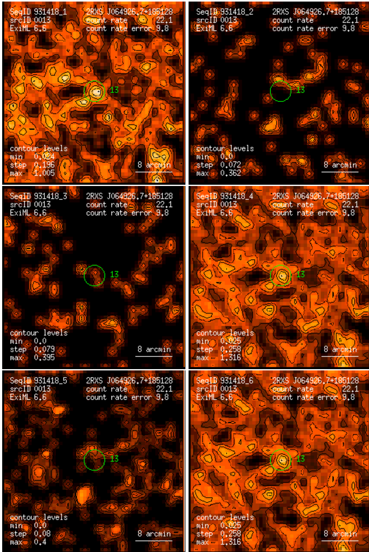
Figure 13: RASS 931418: detection 0013: band rate images, Gaussian filter: (1) PSPC channels 11 – 41, (2) 52 – 90, (3) 91 – 201, (4) 11 – 235, (5) 52 – 201, (6) 11 – 201. Broad band rates in counts/ks. Band rate contour levels in counts/ks/arcmin 2 .
