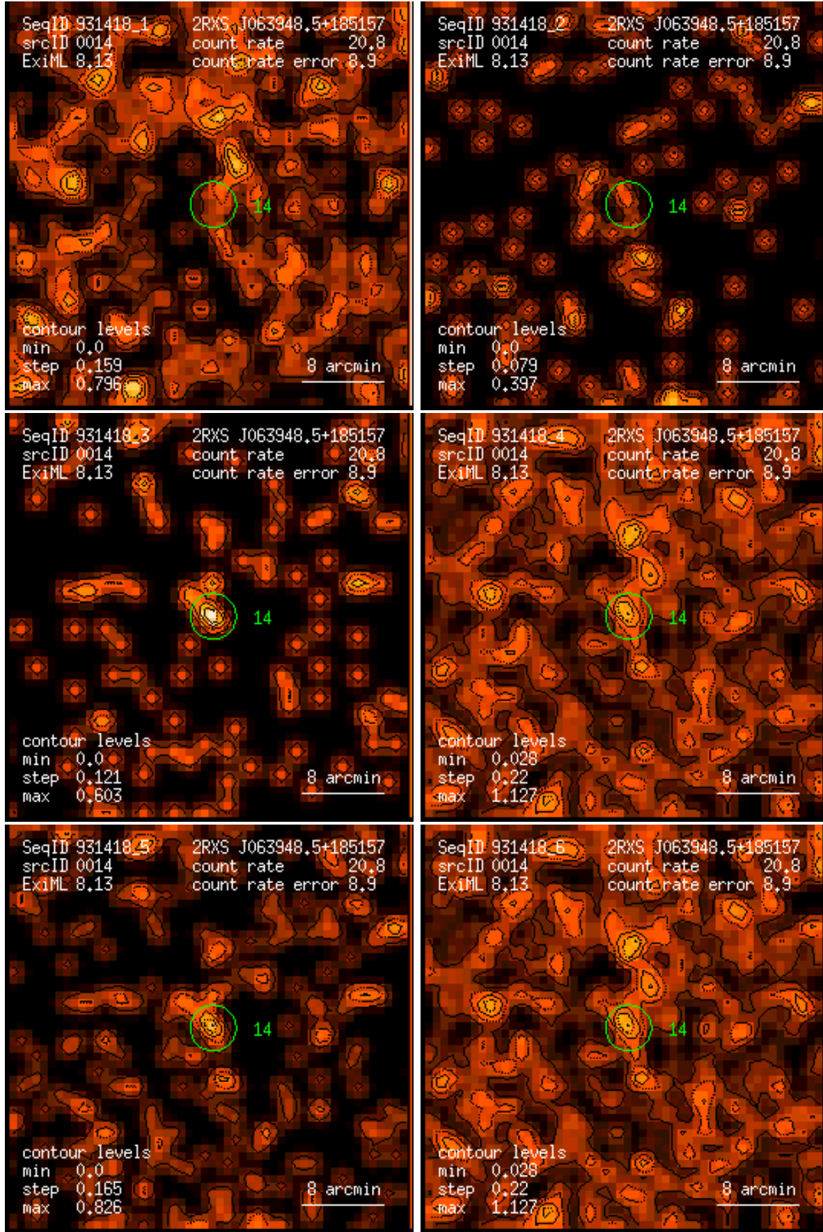
Figure 14: RASS 931418: detection 0014: band rate images, Gaussian filter: (1) PSPC channels 11 – 41, (2) 52 – 90, (3) 91 – 201, (4) 11 – 235, (5) 52 – 201, (6) 11 – 201. Broad band rates in counts/ks. Band rate contour levels in counts/ks/arcmin 2 .
