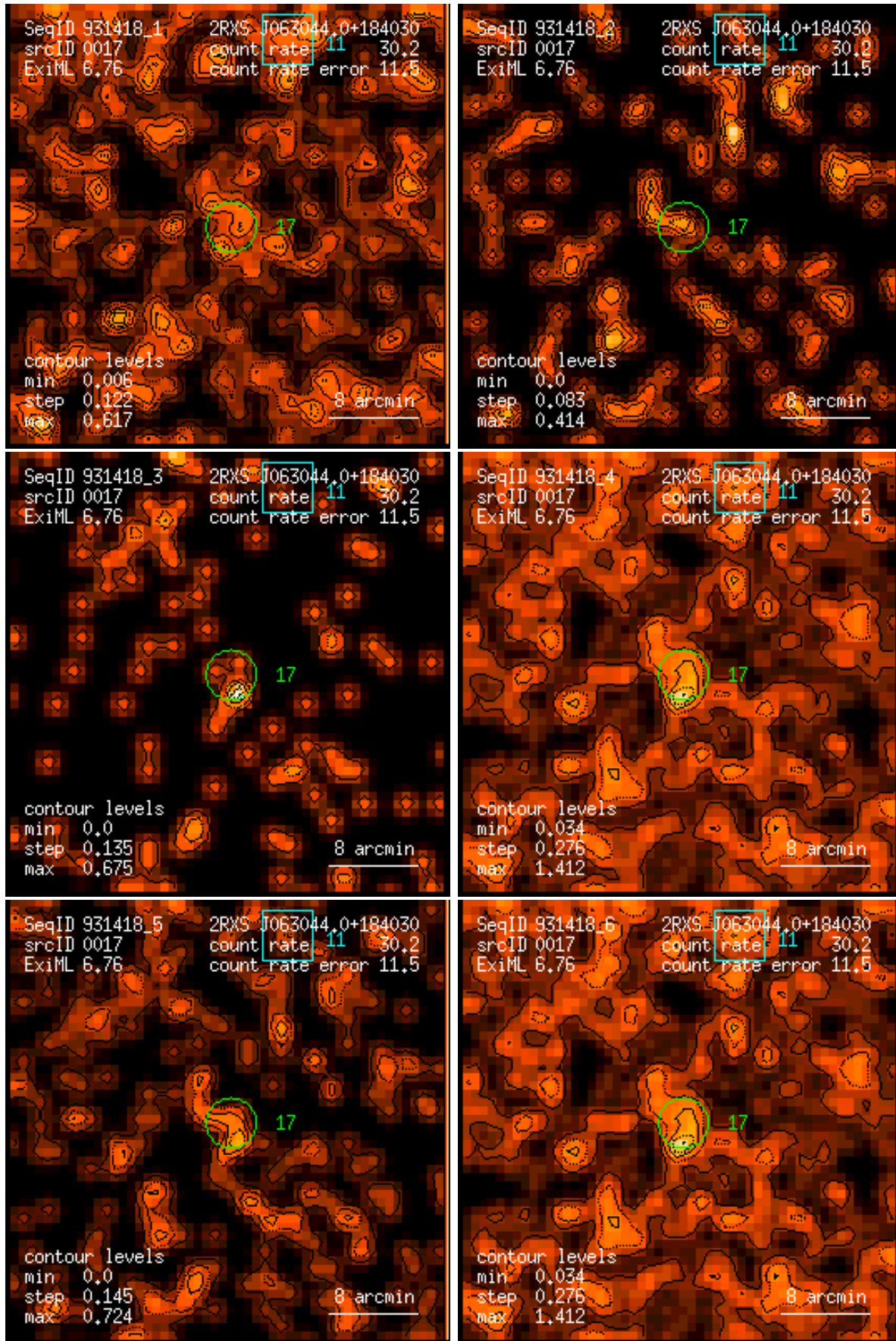
Figure 17: RASS 931418: detection 0017: band rate images, Gaussian filter: (1) PSPC channels 11 – 41, (2) 52 – 90, (3) 91 – 201, (4) 11 – 235, (5) 52 – 201, (6) 11 – 201. Broad band rates in counts/ks. Band rate contour levels in counts/ks/arcmin 2 .
