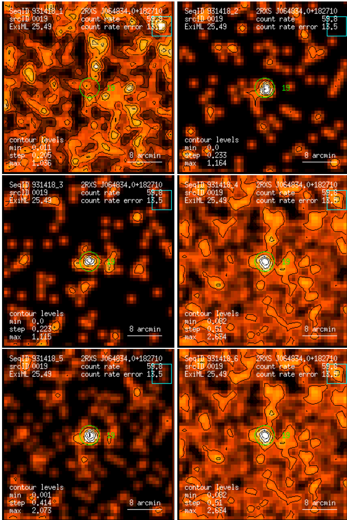
Figure 19: RASS 931418: detection 0019: band rate images, Gaussian filter: (1) PSPC channels 11 – 41, (2) 52 – 90, (3) 91 – 201, (4) 11 – 235, (5) 52 – 201, (6) 11 – 201. Broad band rates in counts/ks. Band rate contour levels in counts/ks/arcmin 2 .
