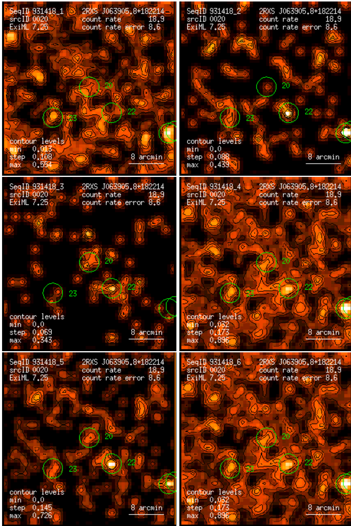
Figure 20: RASS 931418: detection 0020: band rate images, Gaussian filter: (1) PSPC channels 11 – 41, (2) 52 – 90, (3) 91 – 201, (4) 11 – 235, (5) 52 – 201, (6) 11 – 201. Broad band rates in counts/ks. Band rate contour levels in counts/ks/arcmin 2 .
