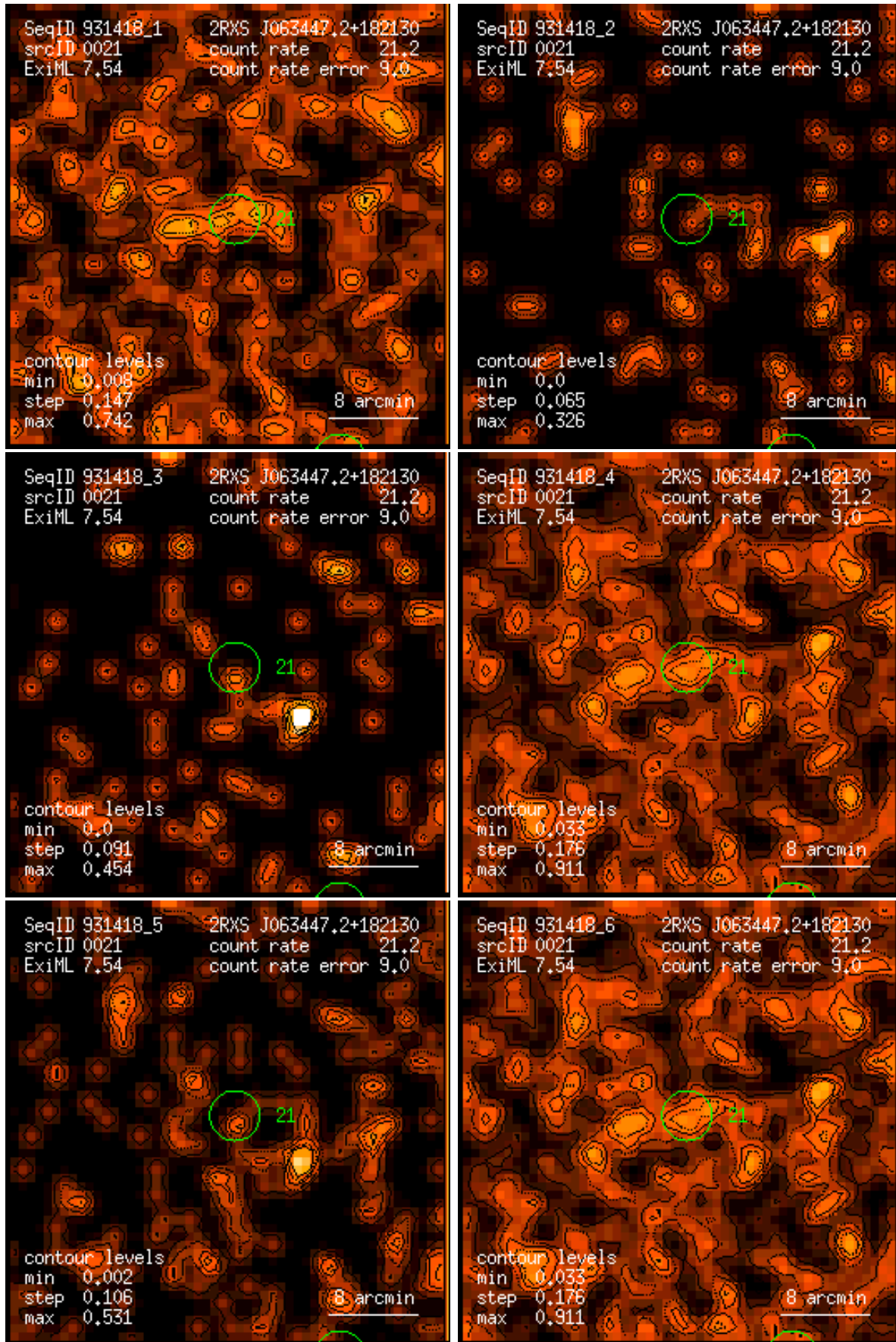
Figure 21: RASS 931418: detection 0021: band rate images, Gaussian filter: (1) PSPC channels 11 – 41, (2) 52 – 90, (3) 91 – 201, (4) 11 – 235, (5) 52 – 201, (6) 11 – 201. Broad band rates in counts/ks. Band rate contour levels in counts/ks/arcmin 2 .
