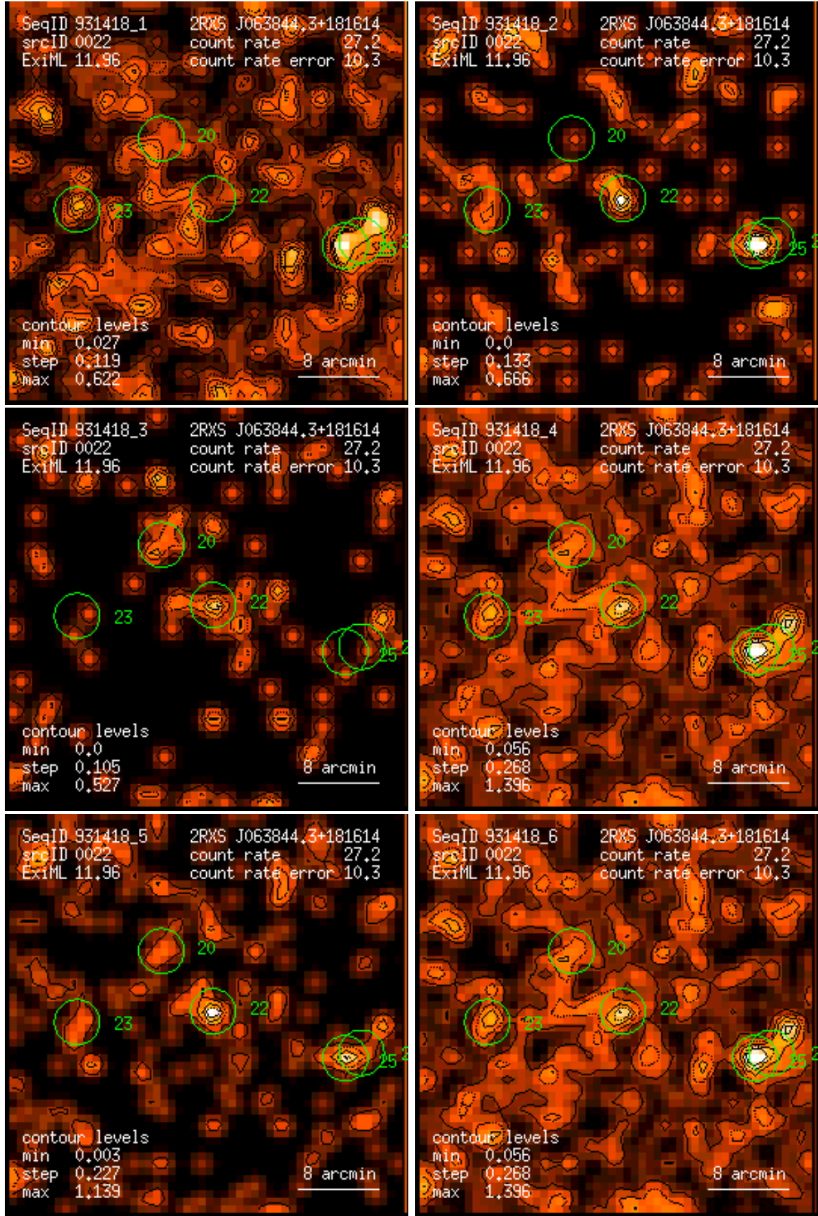
Figure 22: RASS 931418: detection 0022: band rate images, Gaussian filter: (1) PSPC channels 11 – 41, (2) 52 – 90, (3) 91 – 201, (4) 11 – 235, (5) 52 – 201, (6) 11 – 201. Broad band rates in counts/ks. Band rate contour levels in counts/ks/arcmin 2 .
