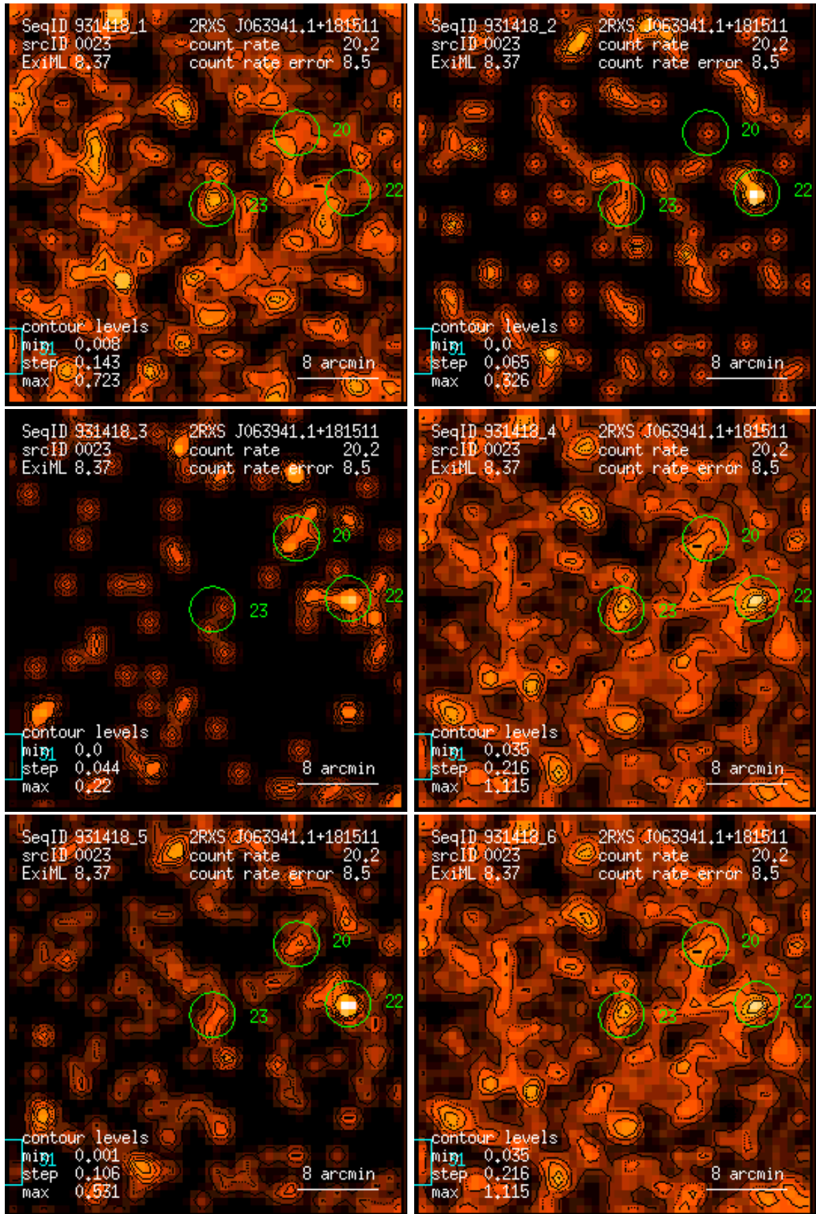
Figure 23: RASS 931418: detection 0023: band rate images, Gaussian filter: (1) PSPC channels 11 – 41, (2) 52 – 90, (3) 91 – 201, (4) 11 – 235, (5) 52 – 201, (6) 11 – 201. Broad band rates in counts/ks. Band rate contour levels in counts/ks/arcmin 2 .
