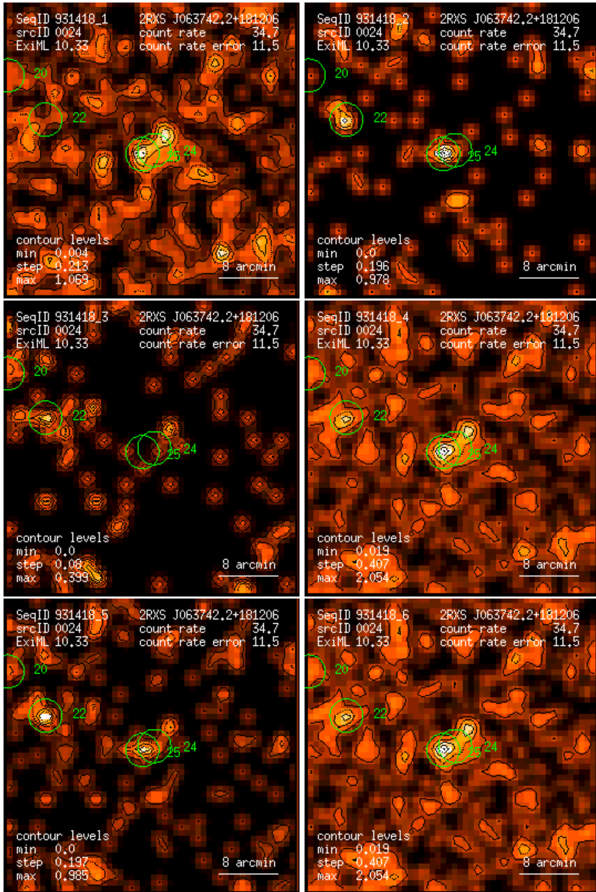
Figure 24: RASS 931418: detection 0024: band rate images, Gaussian filter: (1) PSPC channels 11 – 41, (2) 52 – 90, (3) 91 – 201, (4) 11 – 235, (5) 52 – 201, (6) 11 – 201. Broad band rates in counts/ks. Band rate contour levels in counts/ks/arcmin 2 .
