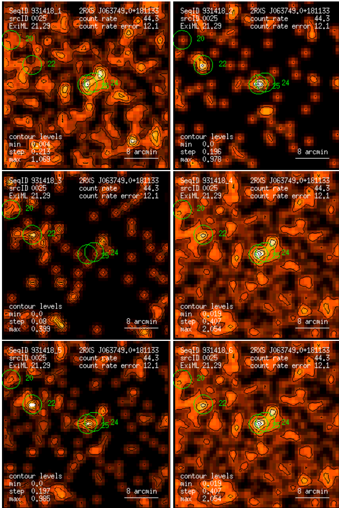
Figure 25: RASS 931418: detection 0025: band rate images, Gaussian filter: (1) PSPC channels 11 – 41, (2) 52 – 90, (3) 91 – 201, (4) 11 – 235, (5) 52 – 201, (6) 11 – 201. Broad band rates in counts/ks. Band rate contour levels in counts/ks/arcmin 2 .
