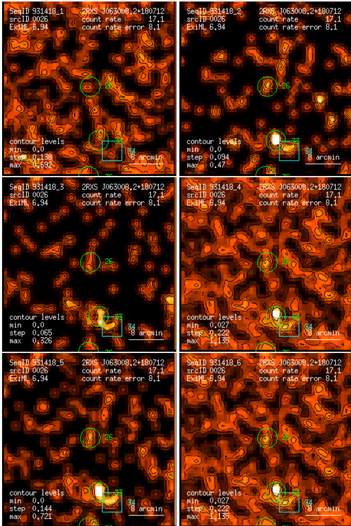
Figure 26: RASS 931418: detection 0026: band rate images, Gaussian filter: (1) PSPC channels 11 – 41, (2) 52 – 90, (3) 91 – 201, (4) 11 – 235, (5) 52 – 201, (6) 11 – 201. Broad band rates in counts/ks. Band rate contour levels in counts/ks/arcmin 2 .
