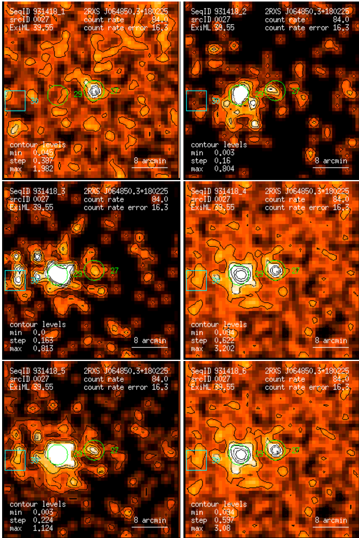
Figure 27: RASS 931418: detection 0027: band rate images, Gaussian filter: (1) PSPC channels 11 – 41, (2) 52 – 90, (3) 91 – 201, (4) 11 – 235, (5) 52 – 201, (6) 11 – 201. Broad band rates in counts/ks. Band rate contour levels in counts/ks/arcmin 2 .
