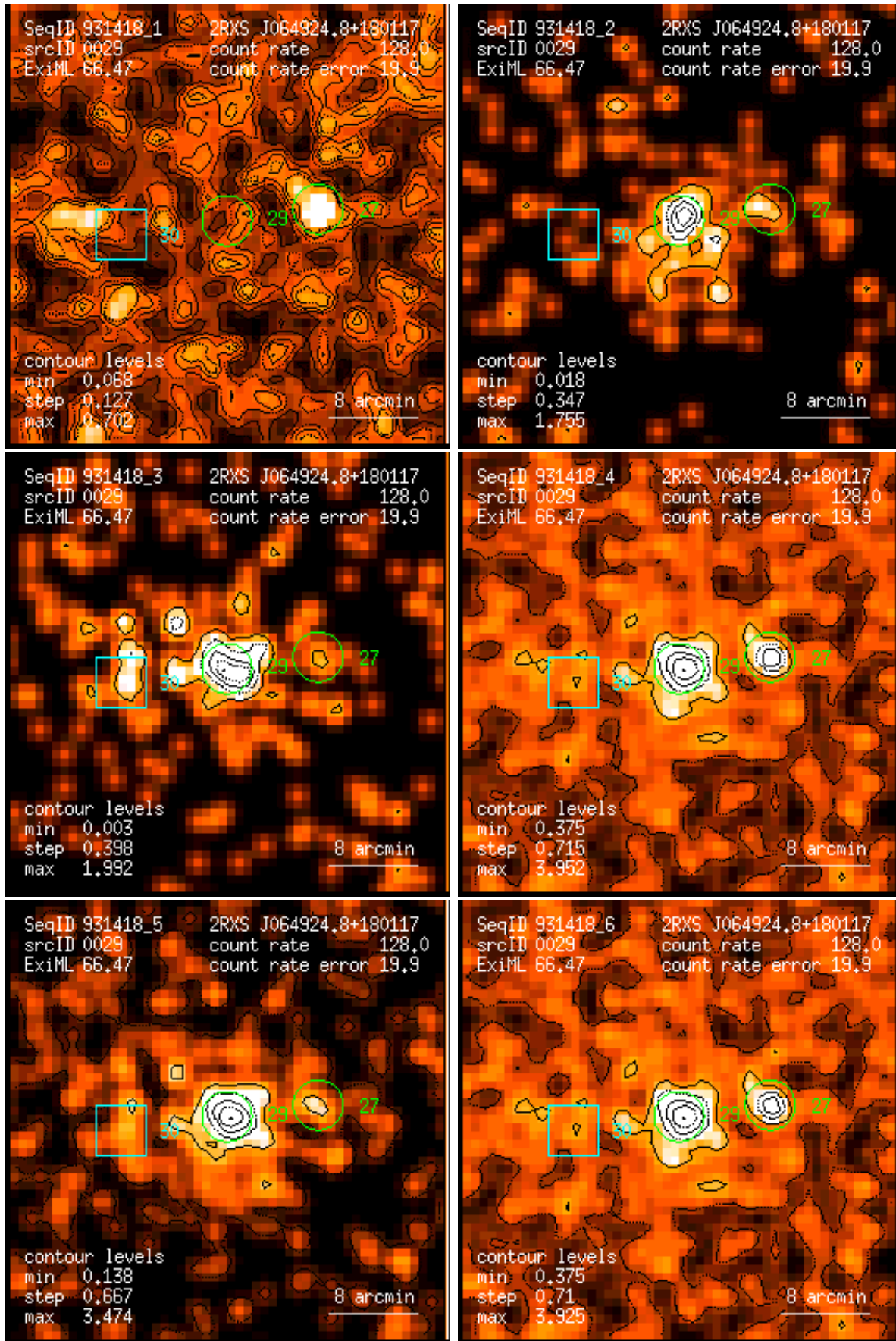
Figure 29: RASS 931418: detection 0029: band rate images, Gaussian filter: (1) PSPC channels 11 – 41, (2) 52 – 90, (3) 91 – 201, (4) 11 – 235, (5) 52 – 201, (6) 11 – 201. Broad band rates in counts/ks. Band rate contour levels in counts/ks/arcmin 2 .
