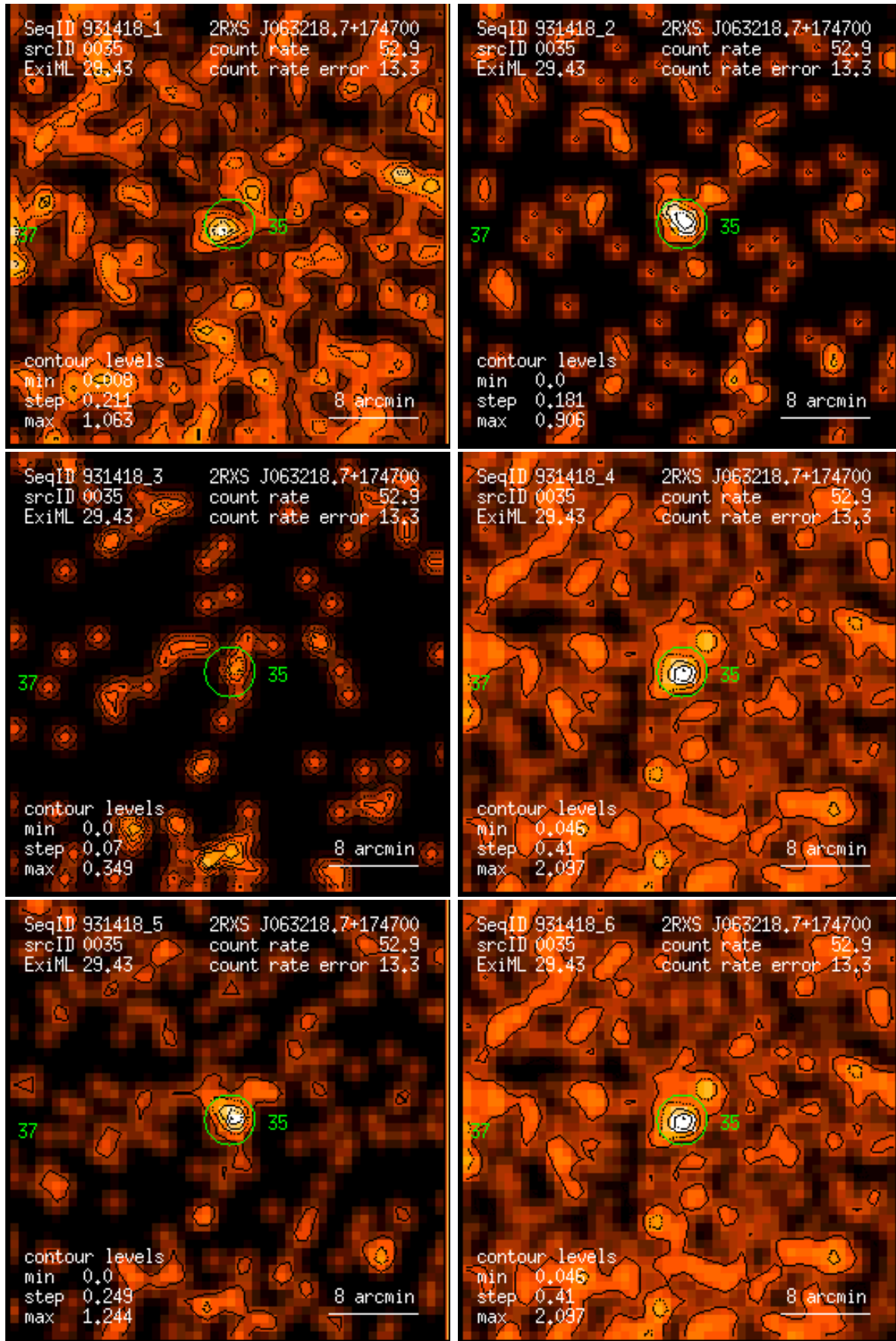
Figure 35: RASS 931418: detection 0035: band rate images, Gaussian filter: (1) PSPC channels 11 – 41, (2) 52 – 90, (3) 91 – 201, (4) 11 – 235, (5) 52 – 201, (6) 11 – 201. Broad band rates in counts/ks. Band rate contour levels in counts/ks/arcmin 2 .
