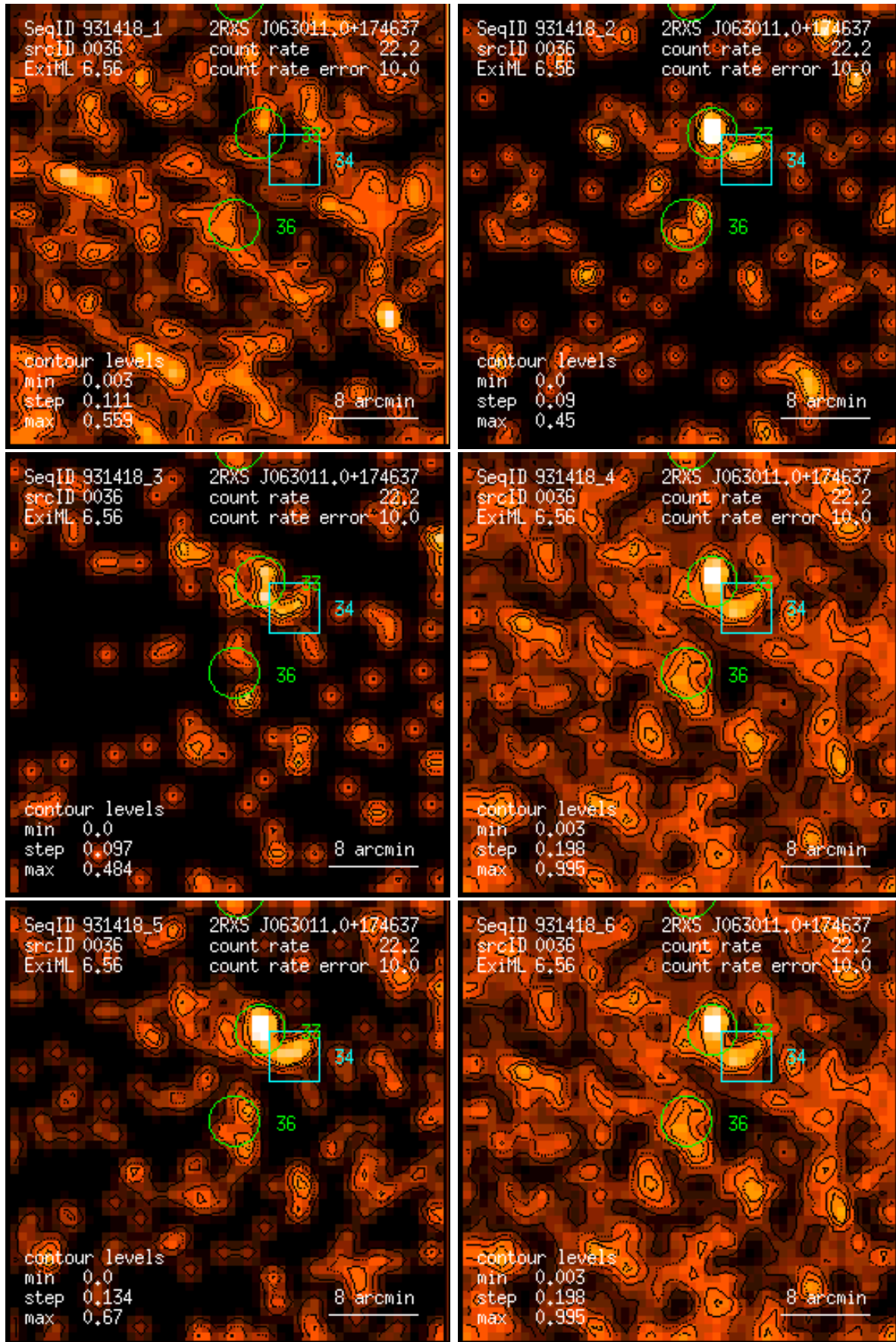
Figure 36: RASS 931418: detection 0036: band rate images, Gaussian filter: (1) PSPC channels 11 – 41, (2) 52 – 90, (3) 91 – 201, (4) 11 – 235, (5) 52 – 201, (6) 11 – 201. Broad band rates in counts/ks. Band rate contour levels in counts/ks/arcmin 2 .
