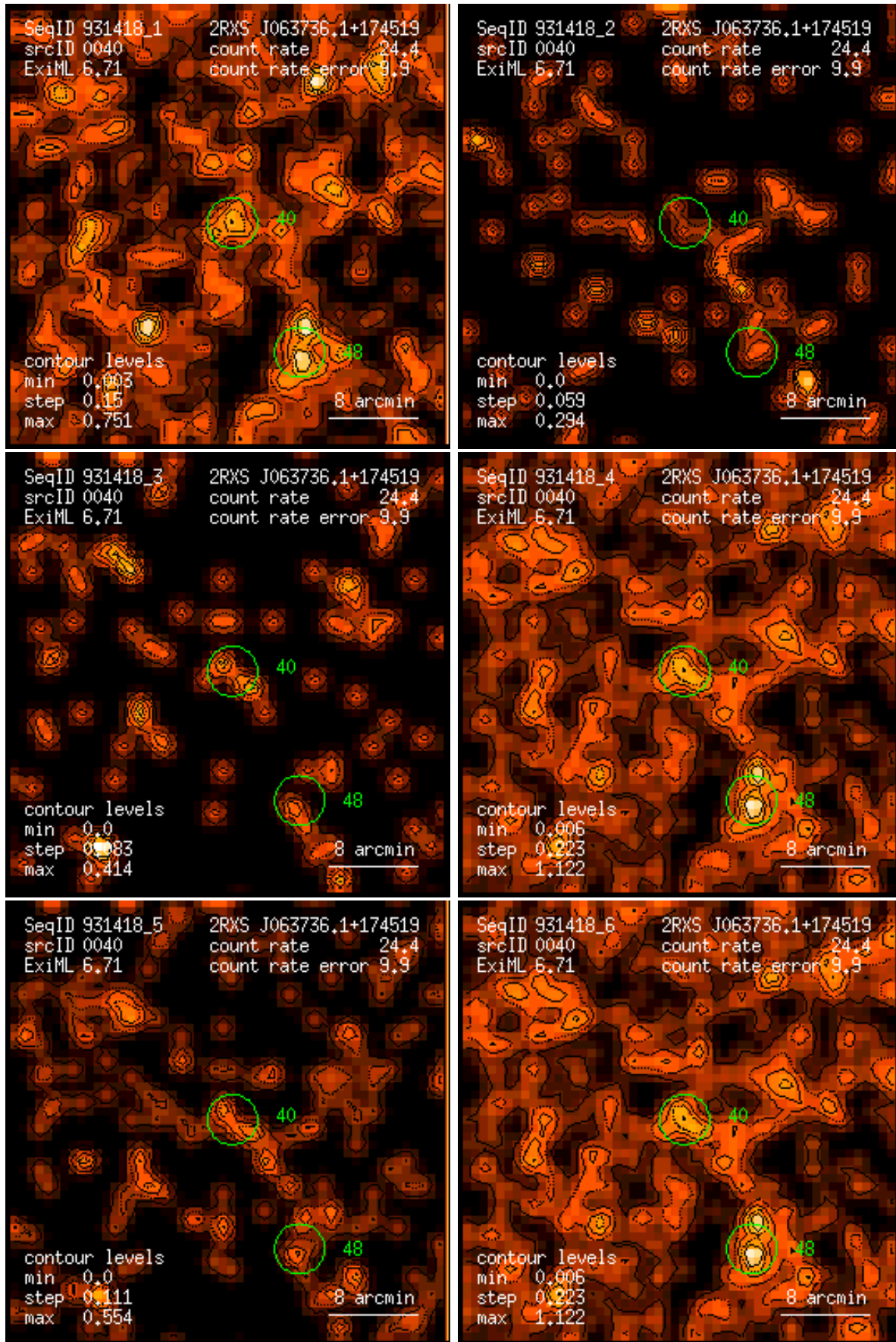
Figure 40: RASS 931418: detection 0040: band rate images, Gaussian filter: (1) PSPC channels 11 – 41, (2) 52 – 90, (3) 91 – 201, (4) 11 – 235, (5) 52 – 201, (6) 11 – 201. Broad band rates in counts/ks. Band rate contour levels in counts/ks/arcmin 2 .
