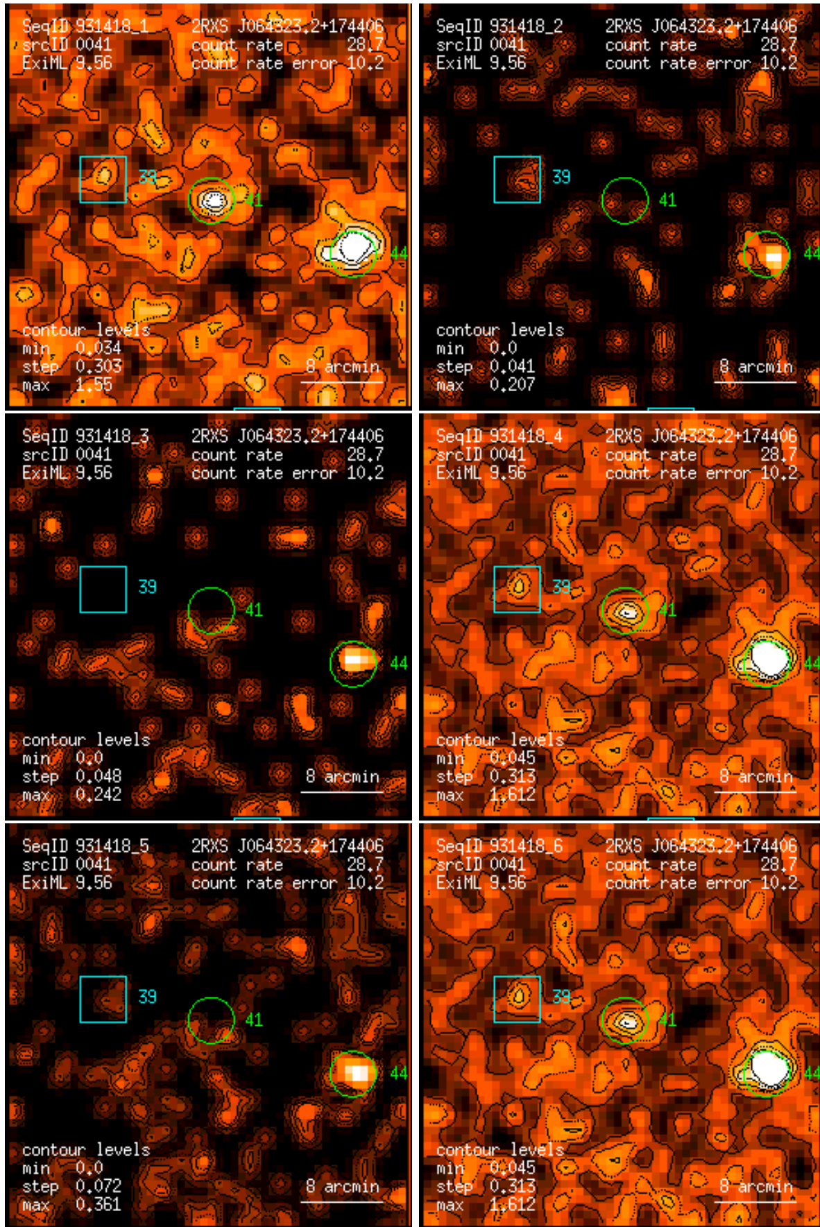
Figure 41: RASS 931418: detection 0041: band rate images, Gaussian filter: (1) PSPC channels 11 – 41, (2) 52 – 90, (3) 91 – 201, (4) 11 – 235, (5) 52 – 201, (6) 11 – 201. Broad band rates in counts/ks. Band rate contour levels in counts/ks/arcmin 2 .
