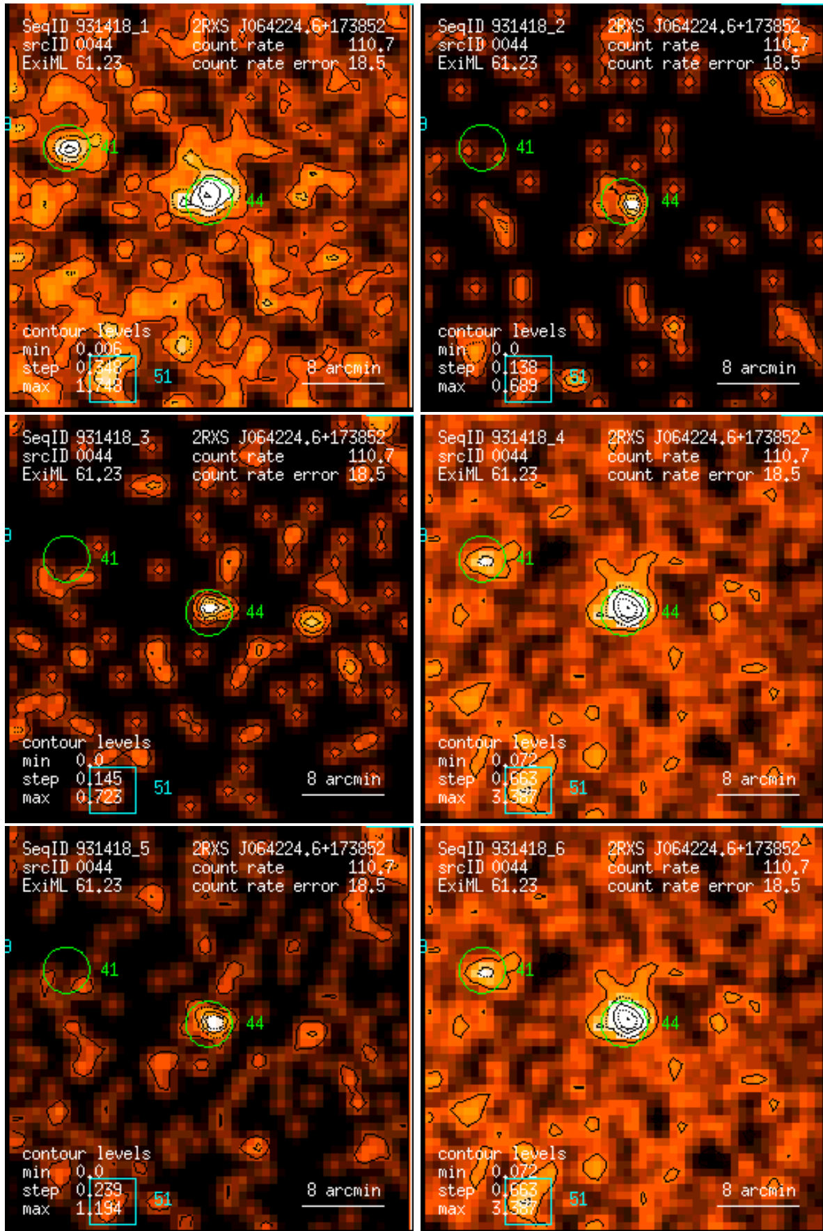
Figure 44: RASS 931418: detection 0044: band rate images, Gaussian filter: (1) PSPC channels 11 – 41, (2) 52 – 90, (3) 91 – 201, (4) 11 – 235, (5) 52 – 201, (6) 11 – 201. Broad band rates in counts/ks. Band rate contour levels in counts/ks/arcmin 2 .
