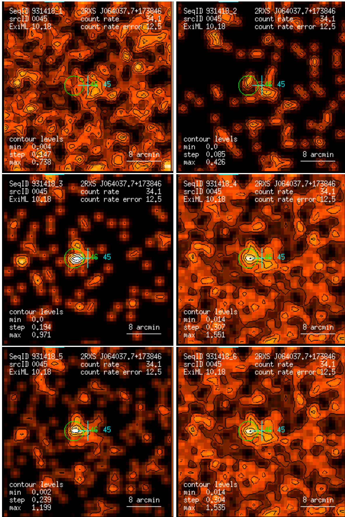
Figure 45: RASS 931418: detection 0045: band rate images, Gaussian filter: (1) PSPC channels 11 – 41, (2) 52 – 90, (3) 91 – 201, (4) 11 – 235, (5) 52 – 201, (6) 11 – 201. Broad band rates in counts/ks. Band rate contour levels in counts/ks/arcmin 2 .
